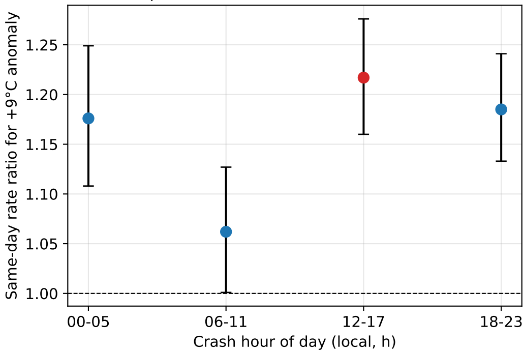
Time-of-day of the heat excess (peak in the hottest hours, 12-17)
