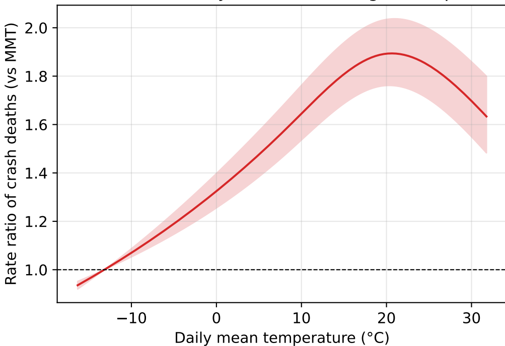
A. Absolute-temperature exposure-response (confounded by seasonal driving envelope)
