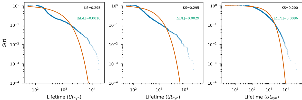
3D Dissipative ( c=100 )
