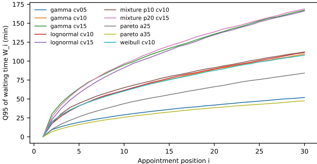
Finite-session delay propagation under fixed slots ( x = E[S] )
