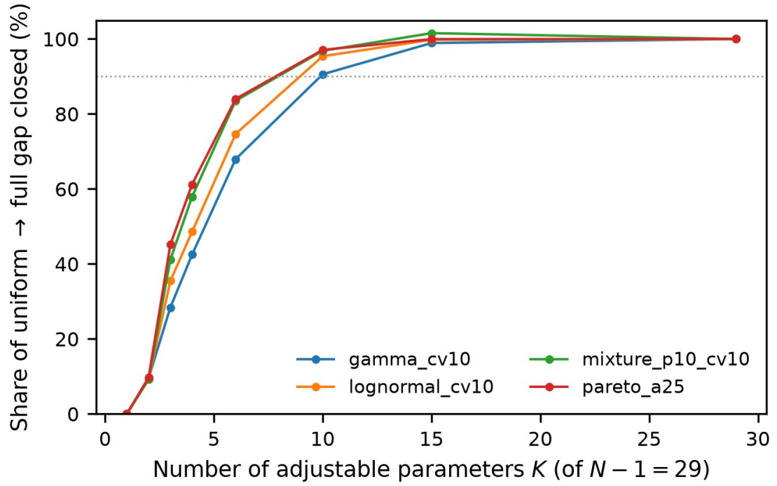
Figure 9. Complexity frontier: share of the uniform-to-full gap closed by K piecewise-constant blocks ( N=30 , CV = 1.0 , four families).
