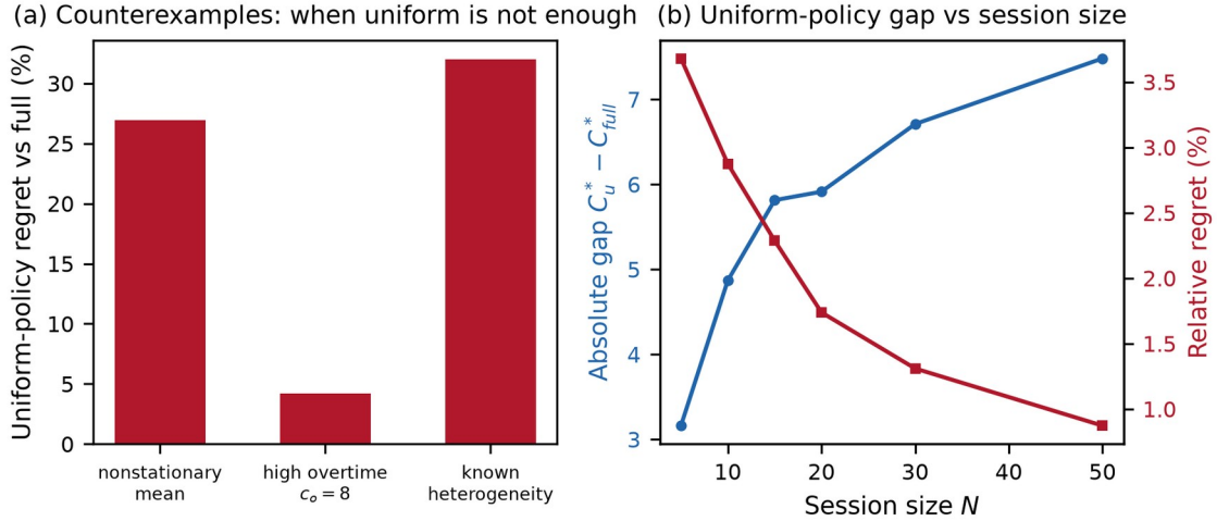
Figure 11. (a) Uniform-policy regret vs full design under nonstationary service, high overtime weight, and known heterogeneity. (b) Absolute gap and relative regret vs session size N .
