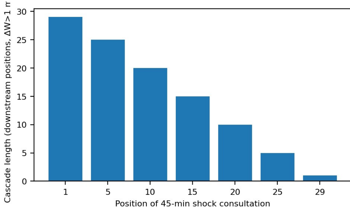
Figure 7. Delay cascade from a single injected 45-min consultation; cascade length counts downstream appointments with > 1 \text{ min} added waiting.
