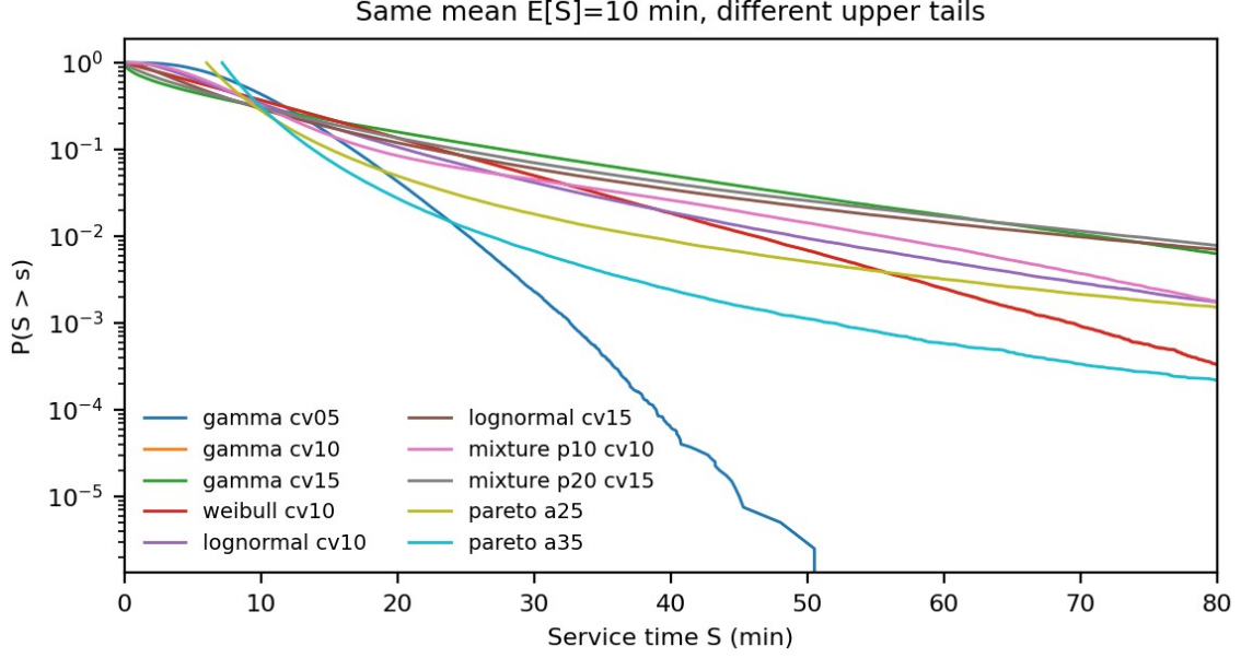
Figure 1. Same-mean ( E[S] = 10 min) service-time distributions with different upper tails (survival functions).
