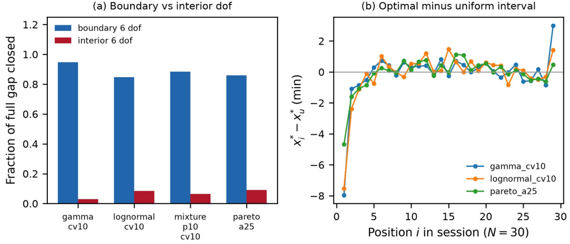
Figure 10. (a) Fraction of the full nonuniform gap closed by six boundary (first/last three) vs six interior degrees of freedom ( N = 30 ). (b) Optimal interval minus uniform interval by session position.
