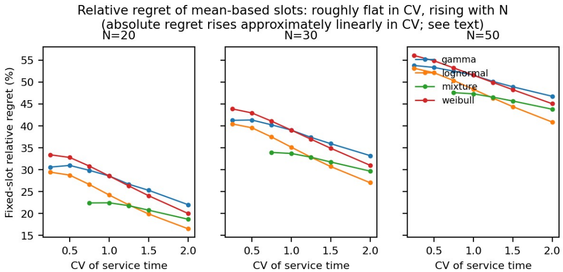
Figure 3. Fixed mean-based slot relative regret across families and CV, by session size N .
