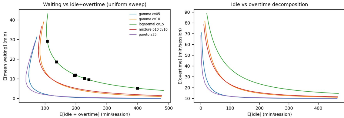
Figure 6. Waiting vs idle+overtime trade-off under the uniform-interval sweep.
