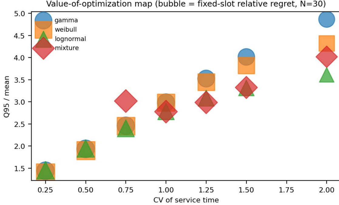
Figure 8. Value-of-optimization map (bubble size = fixed-slot relative regret, N = 30 ).
