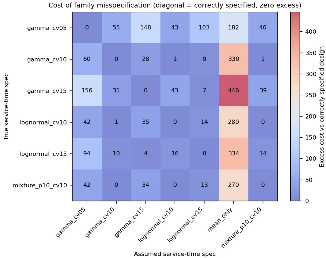
Figure 4. True x assumed distribution matrix: excess cost of misspecification.
