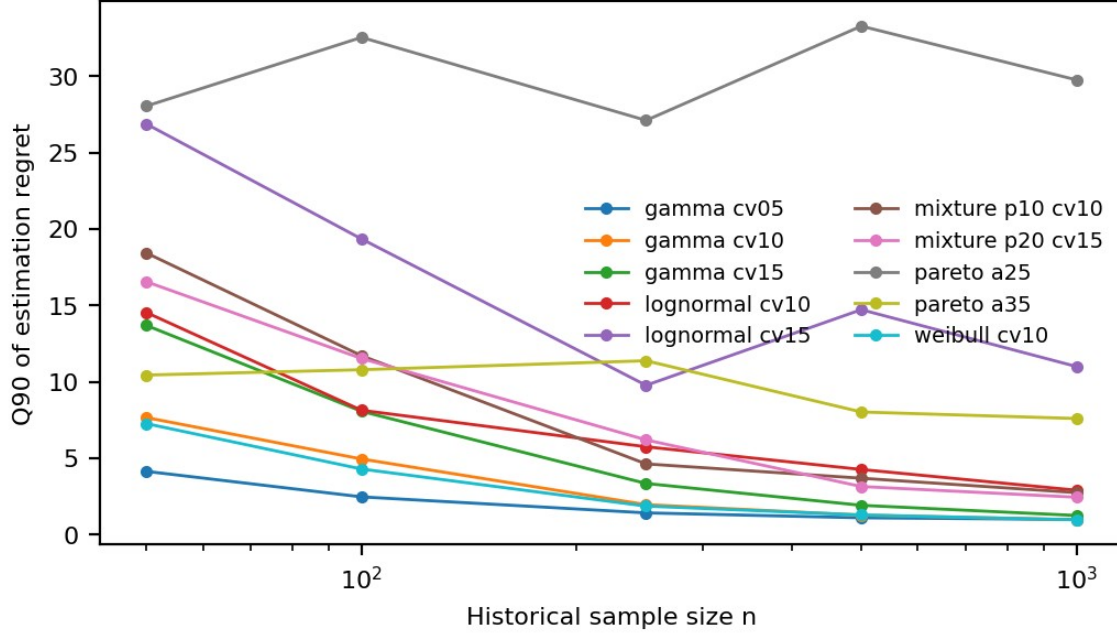
Figure 5. Moment-fitted gamma design regret vs historical sample size n : Q_{90} regret over 400 replications per cell.
