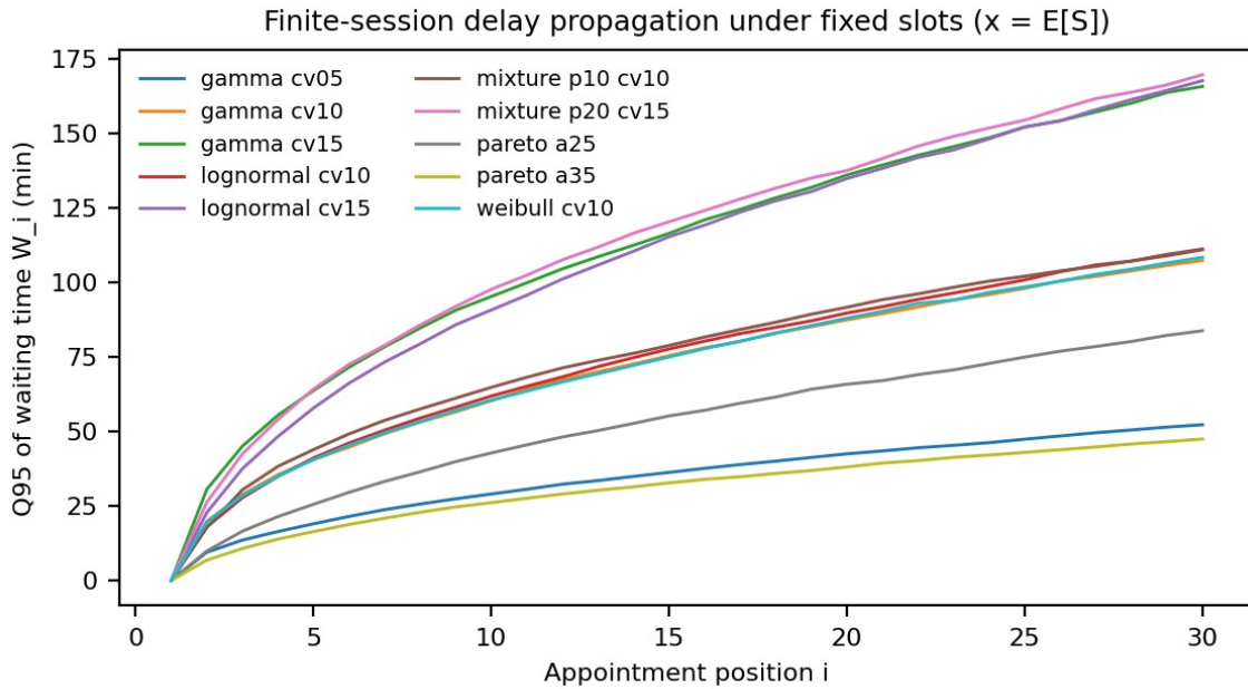
Figure 2. Finite-session delay propagation under fixed mean-based slots ( x = E[S] ).
