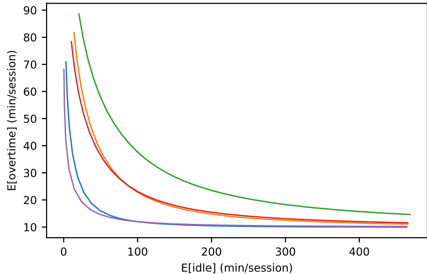
Idle vs overtime decomposition
