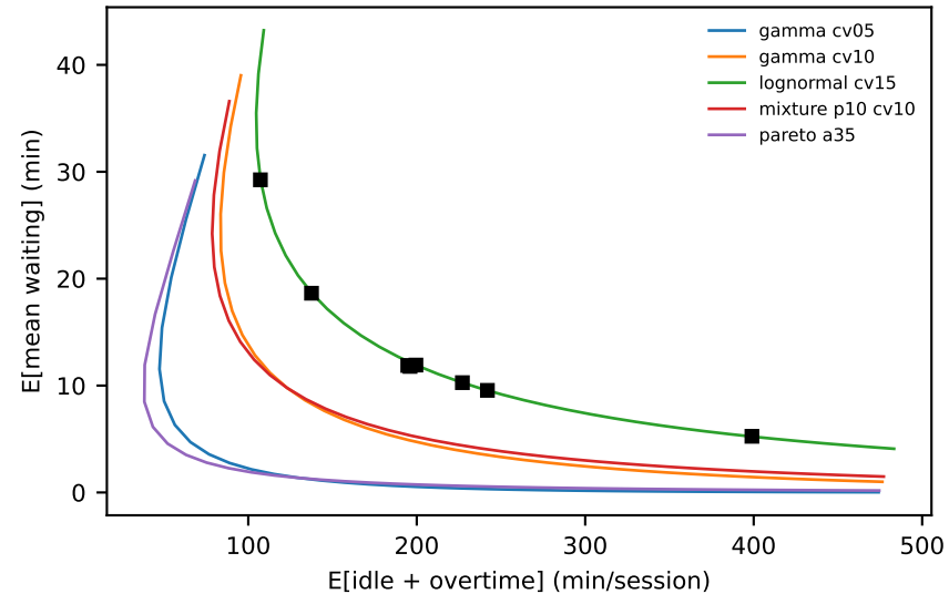
Waiting vs idle+overtime (uniform sweep)
