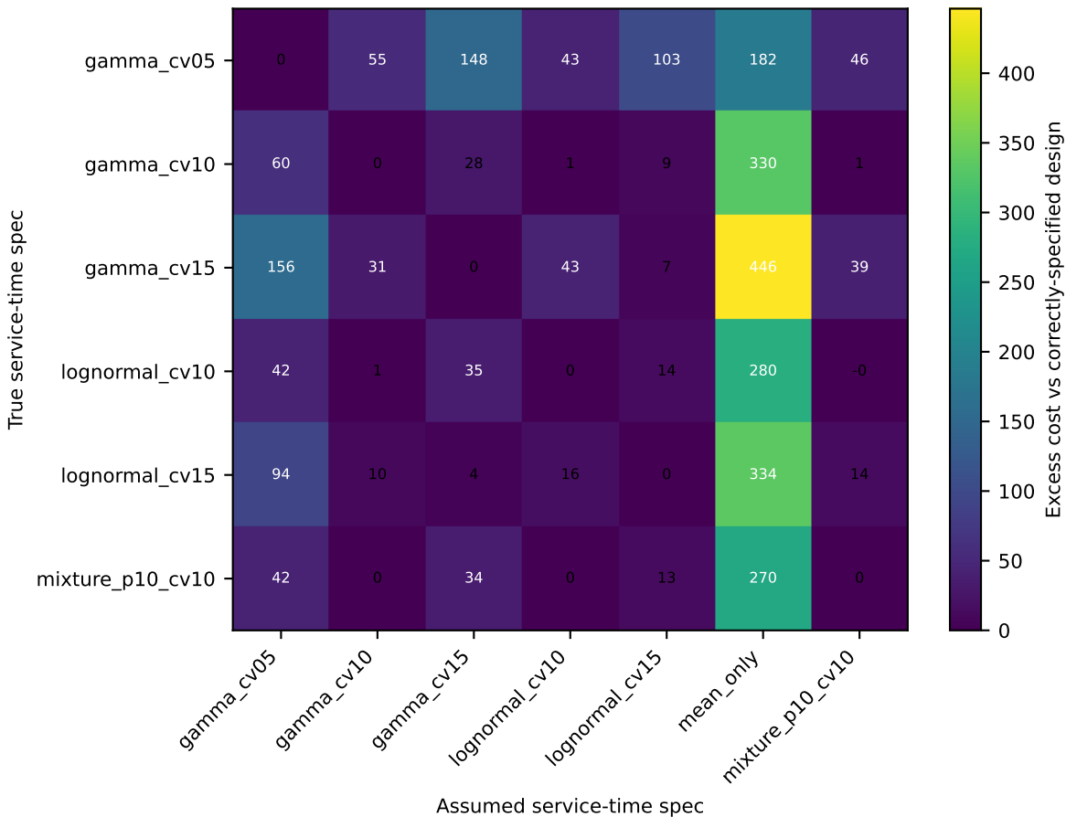
Cost of family misspecification (diagonal = correctly specified, zero excess)
