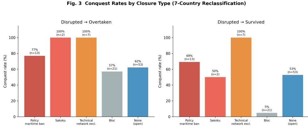
Fig. 3 Conquest rates by closure type under the 7-country reclassification scenario.
