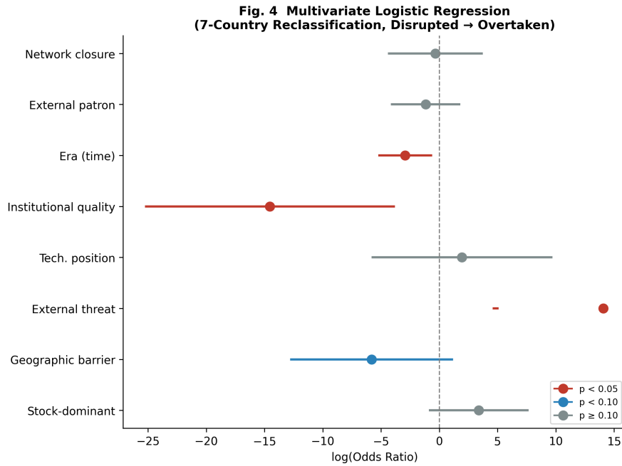
Fig. 4 Forest plot of multivariate logistic regression odds ratios (7-country reclassification, disrupted → overtaken).
