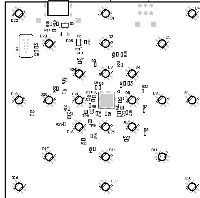
Bottom View (Scale 1:1)
