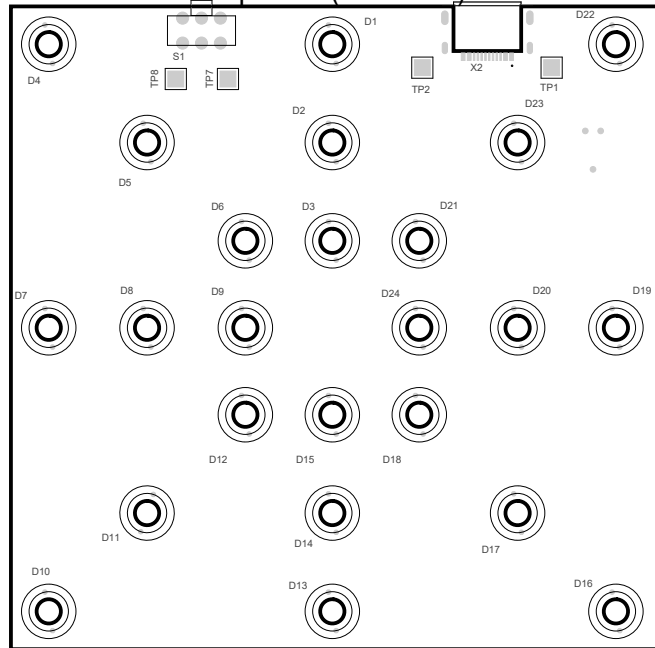
Top View (Scale 1:1)
