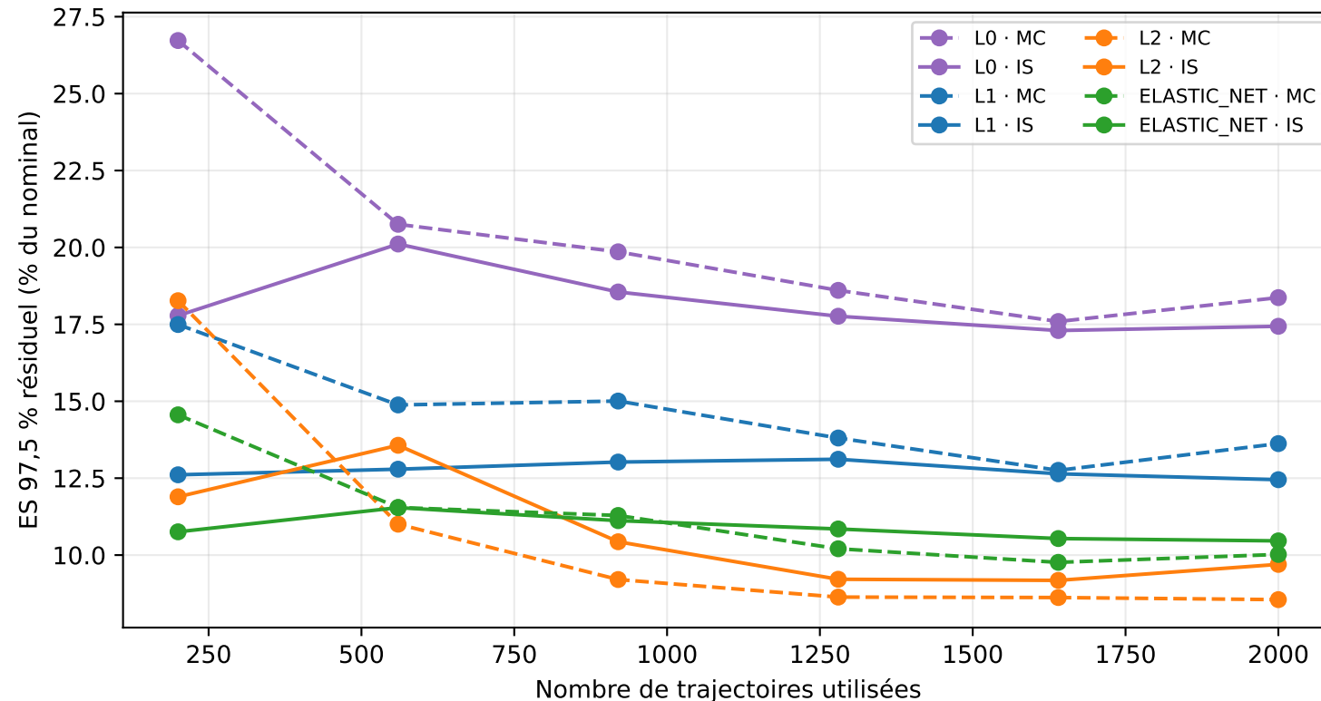
Calls + Puts
