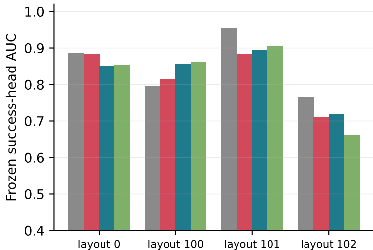
PointMaze: held-out maze layouts (diverse model)
