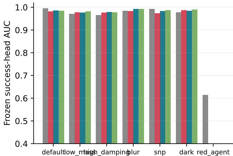
PointMaze: dynamics / visual shifts
