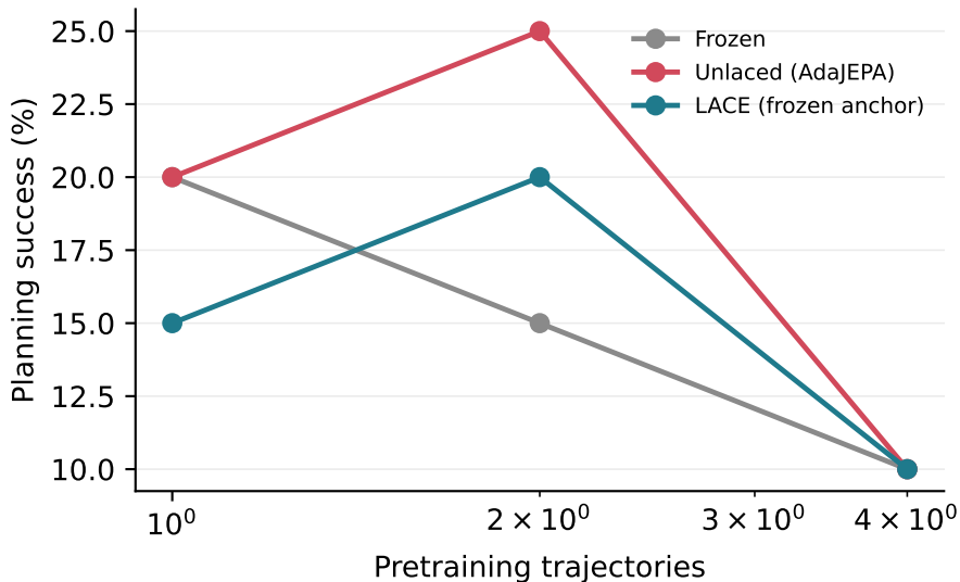
E5: low-data regime (unseen shapes)
