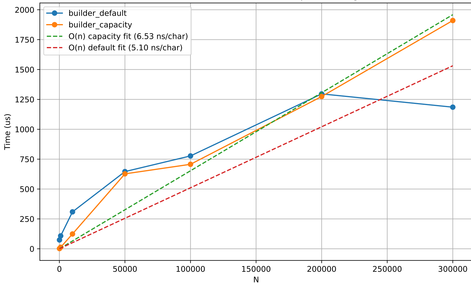
Execution Time vs. N for Linear Repeat Strategies
