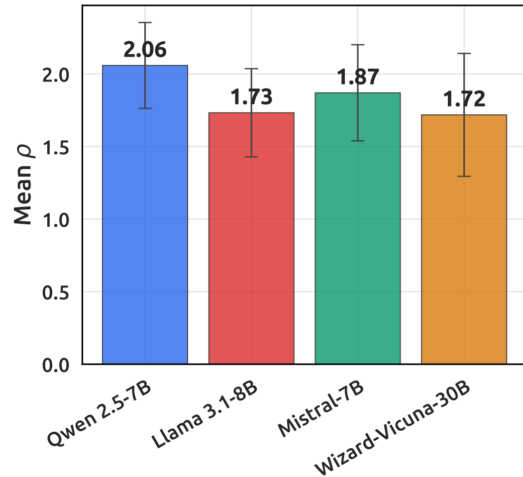
(c) Mean Spectral Gap
