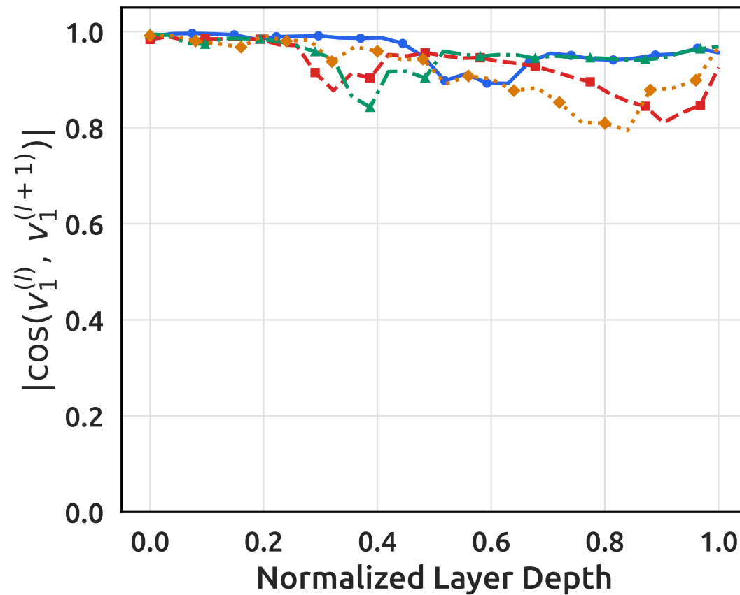
(b) Concept-Spectral Alignment
