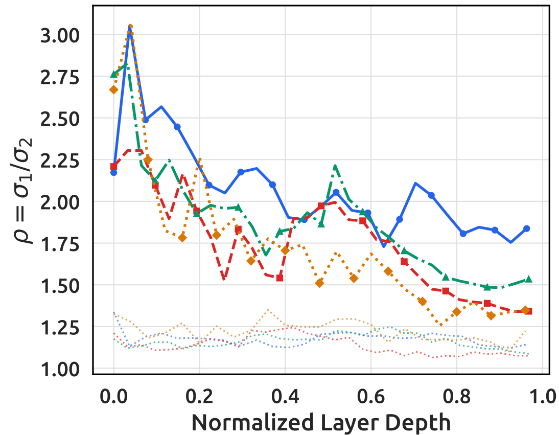
(a) Spectral Gap of D(l)
