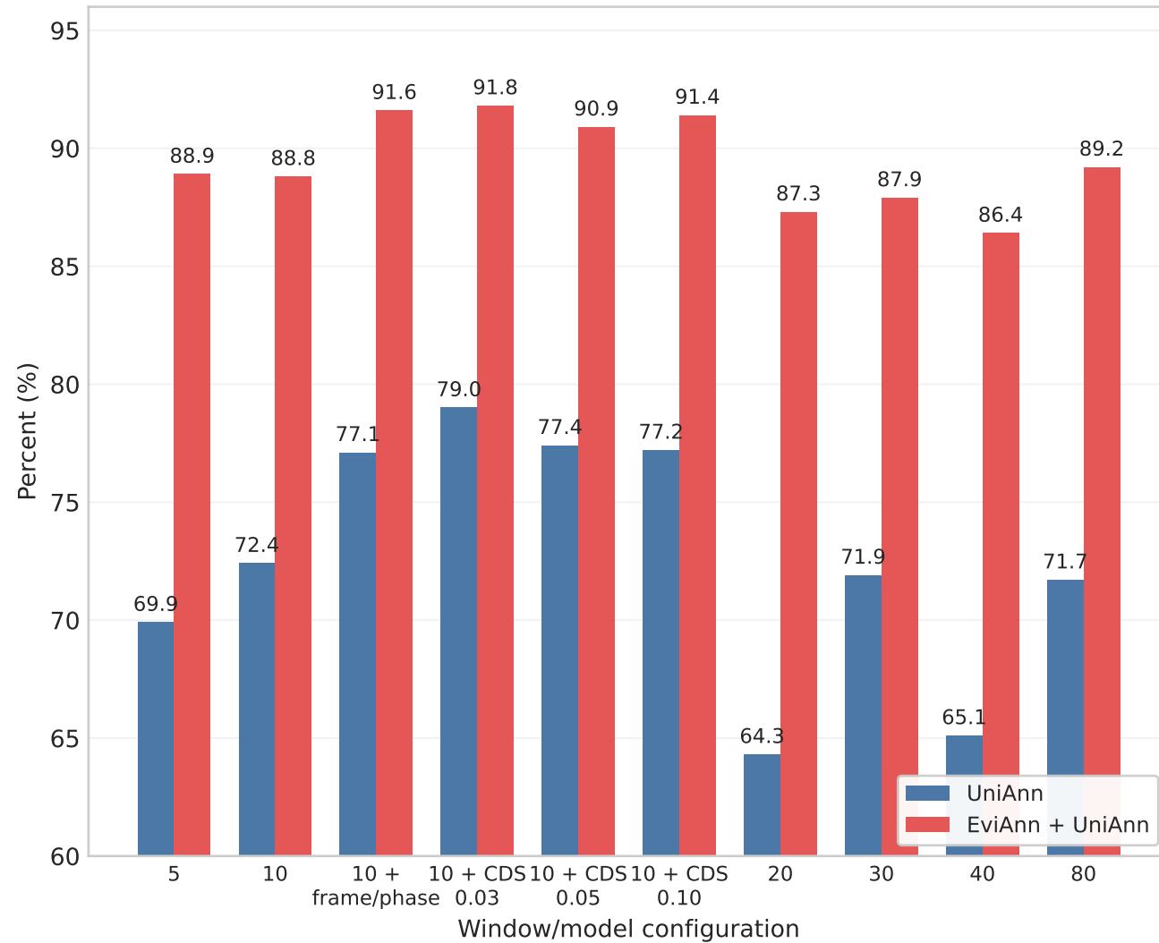
Locus sensitivity
