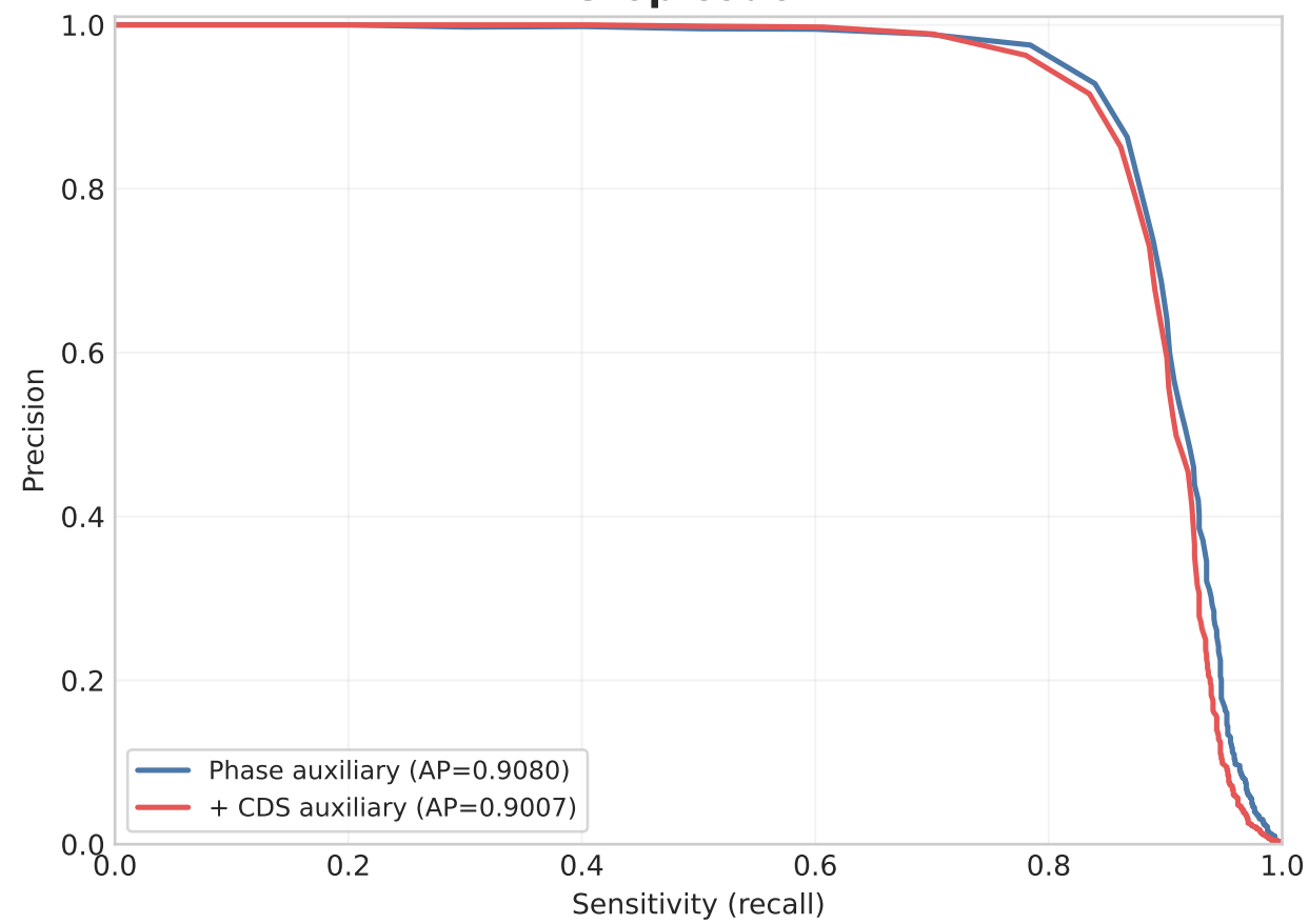
Stop codon
