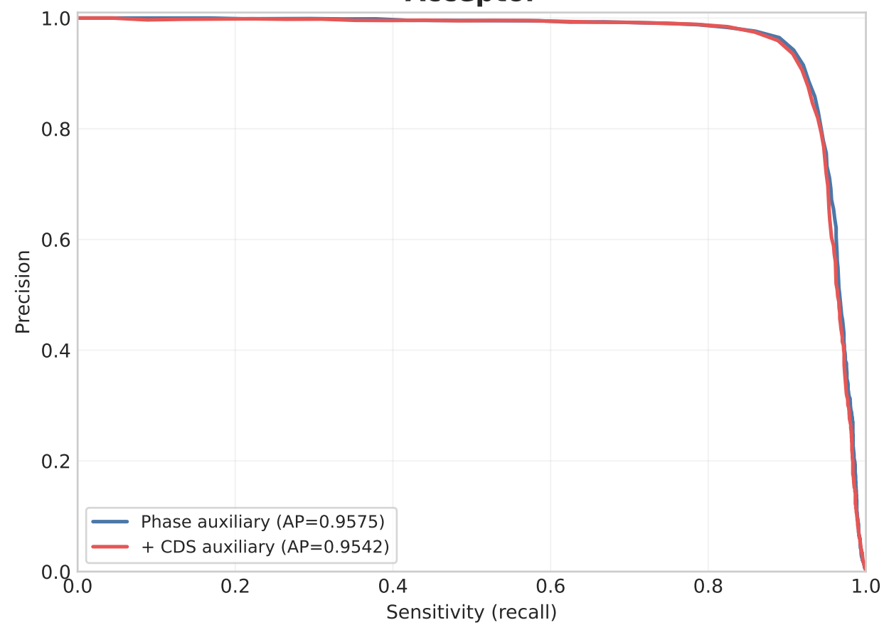
Acceptor
