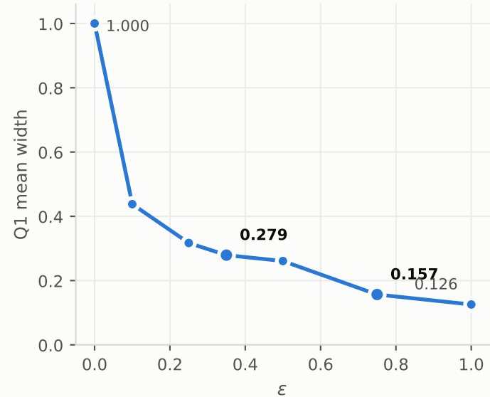
Exact identified-set width
