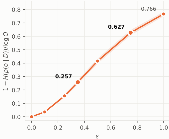
Order-marginal entropy deficit
