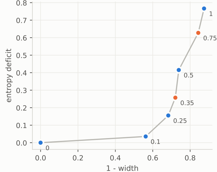
The two axes agree (rank \rho = 1.000 )
