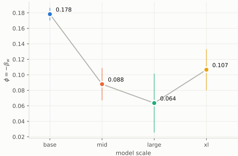
Scale at dose 12000 (step-matched, not compute-matched)
