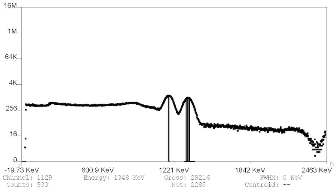
Figure 5: Gamma-ray spectrum of ^{60}\text{Co} collected with the MCA using Amp-to-Direct configuration.
