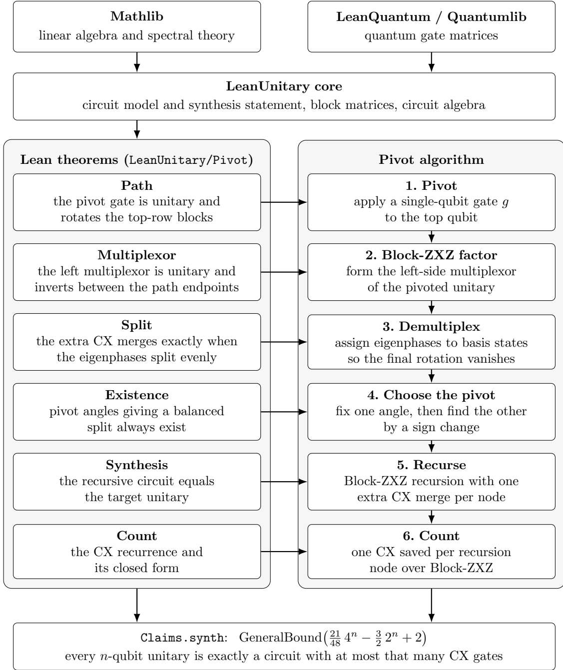
Figure 1: Lean formalization of our proposed pivot decomposition. Each theorem module on the left verifies the step of the pivot algorithm on its right using Mathlib’s linear algebra and the circuit model of LeanUnitary.
