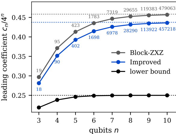
(a) CX count
