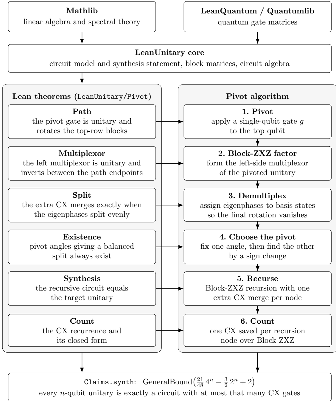
Figure 1: Lean formalization of our proposed pivot decomposition. Each theorem module on the left verifies the step of the pivot algorithm on its right, on top of Mathlib’s linear algebra and the circuit model of LeanUnitary. Together they give the CX bound stated in Claims.synth .
