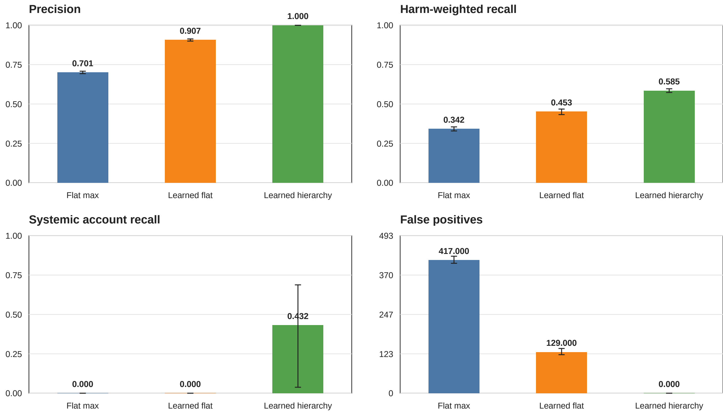
Figure 1. Held-out account review performance at 15% review budget
