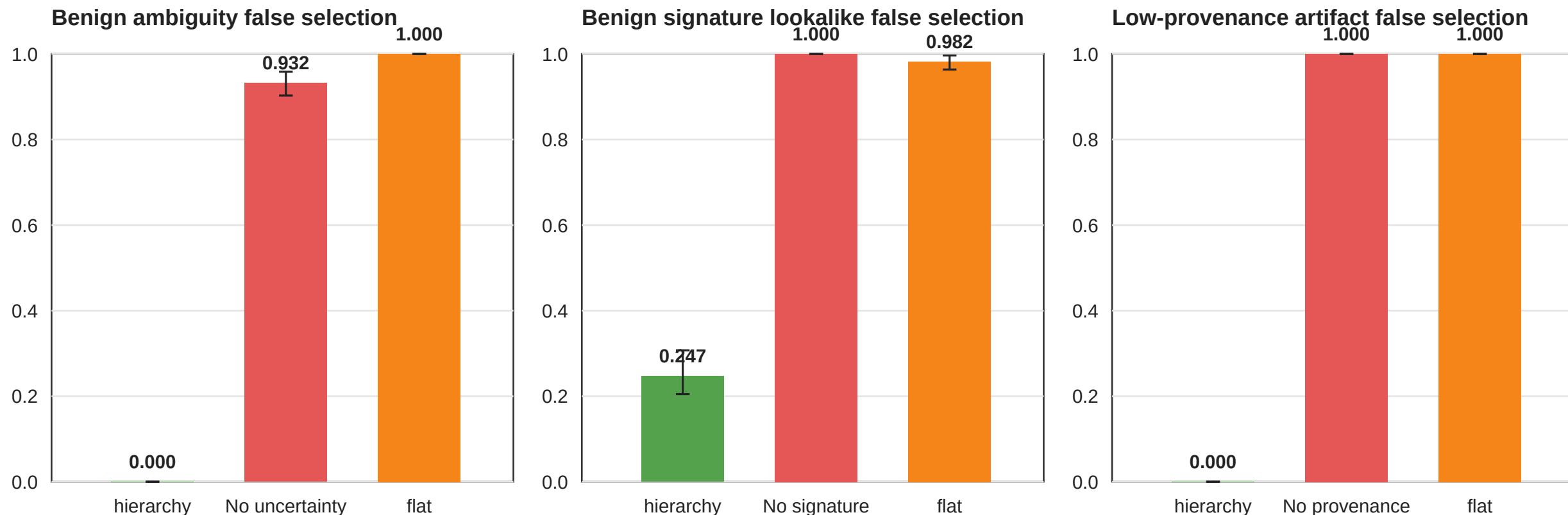
Figure 2. Targeted ablations expose distinct hierarchical-state failure modes
