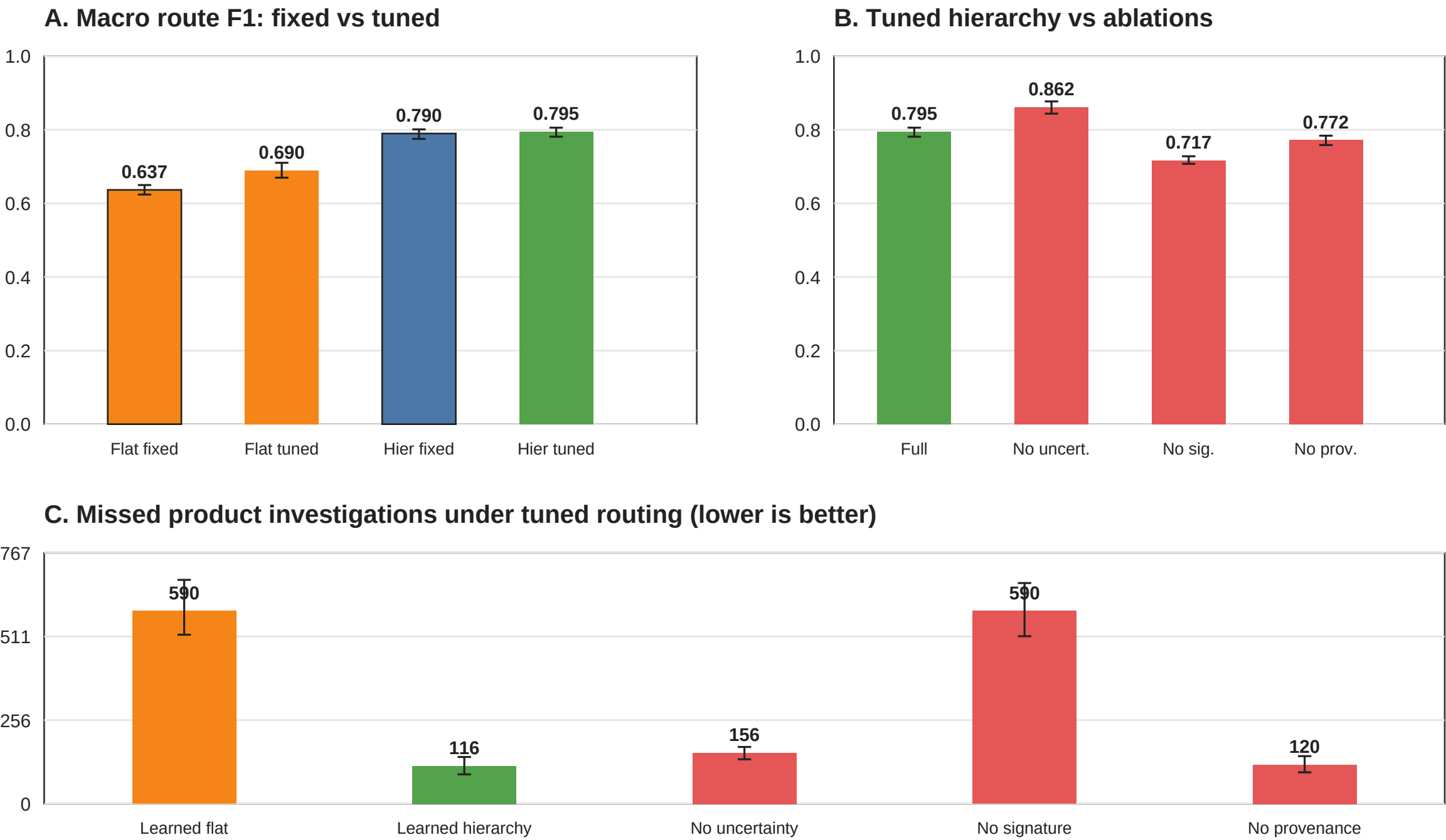
Figure 4. Validation-tuned routing and escalation quality
