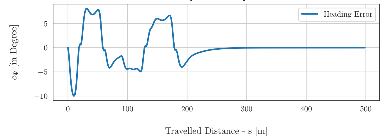
Heading Error e_\psi [in Degree] - With Obstacles
