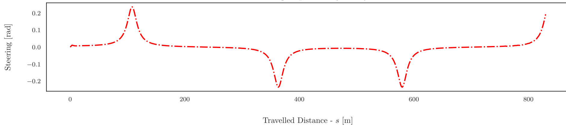
Steering Input Trajectory
