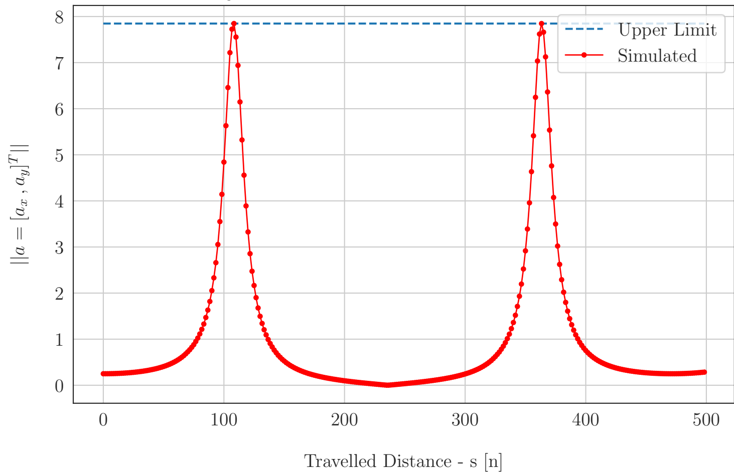
\|a = [a_x, a_y]^T\| Acceleration and Road Adhesion Constraints
