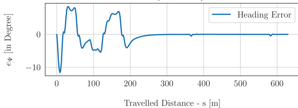
Heading Error e_\psi [in Degree] - No Obstacle
