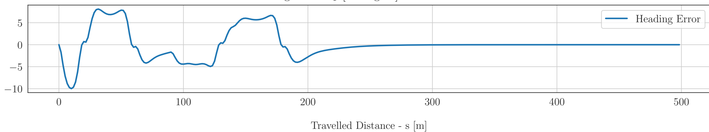
Heading Error e_\psi [in Degree] - With Obstacles
