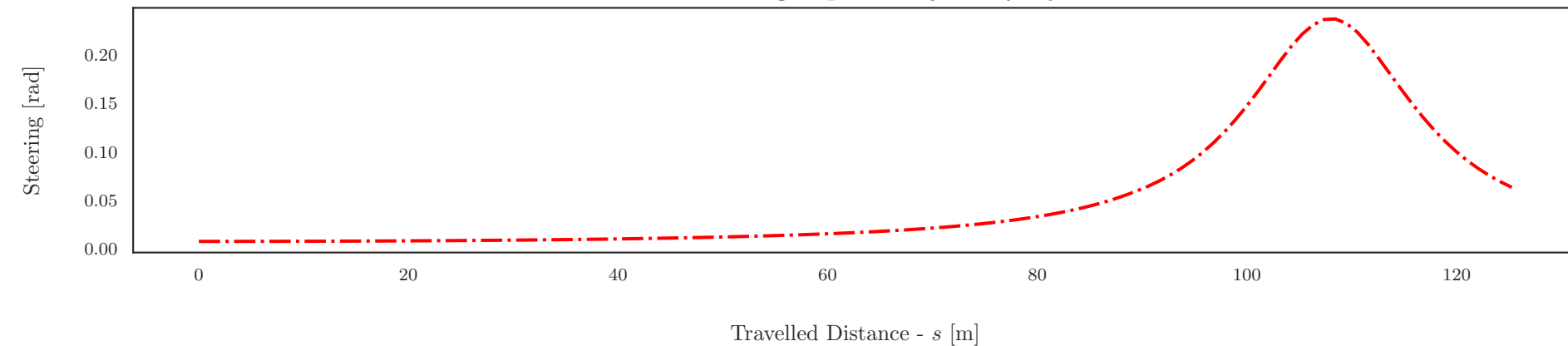
Evolution of Steering Input Trajectory by Iterations
