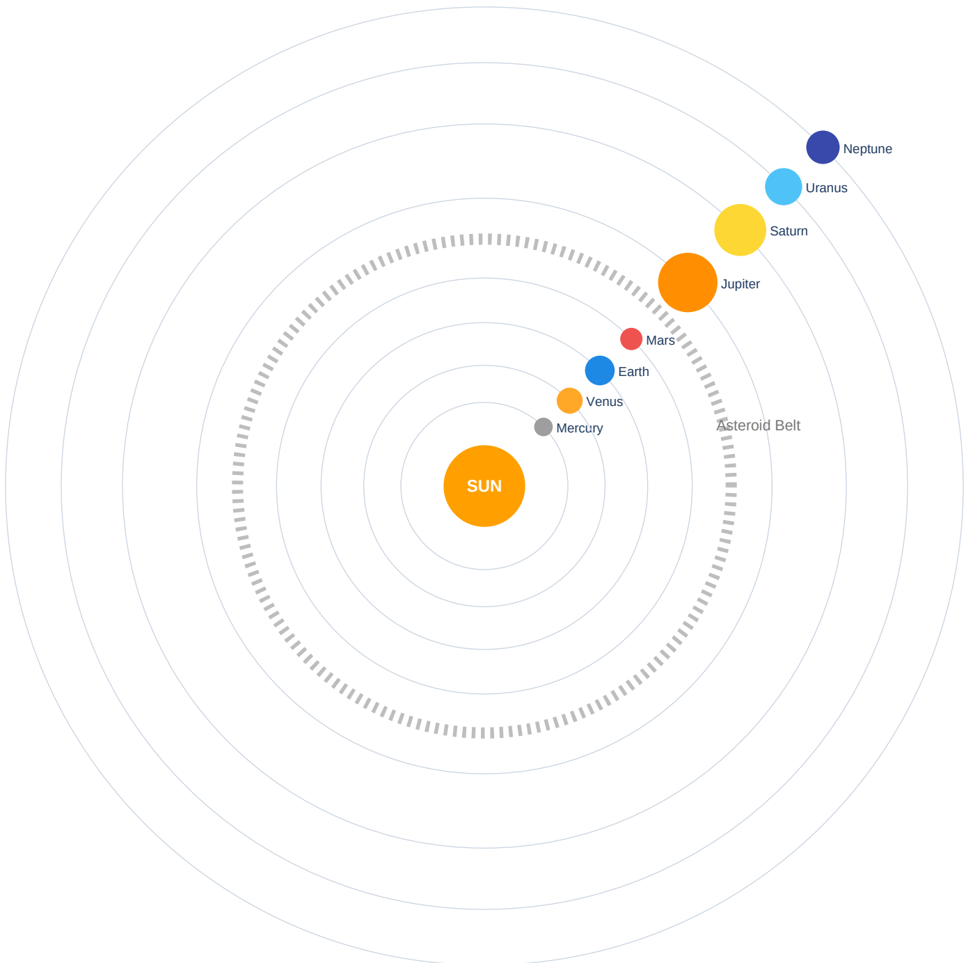
Figure 2: Simplified orbital diagram. Distances and sizes are not to actual scale.
