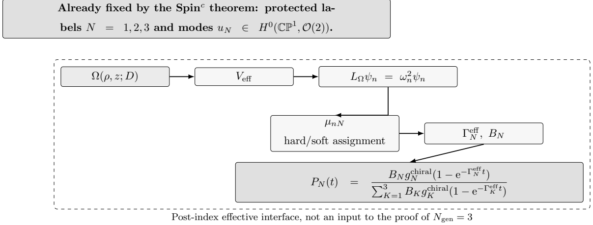
FIG. 6. Post-index scalar spectral interface for formation and visibility. After the \text{Spin}^c index theorem has fixed the protected generation space to three modes, the two-center scalar geometry supplies an effective interface for profiles, rates, and visible overlaps. The conformal factor \Omega determines V_{\text{eff}} , whose scalar eigenmodes \psi_n are connected to the protected labels only through scalarization weights and hard/soft assignment. The probability law P_N(t) describes post-index formation and visibility of N = 1, 2, 3 ; it is not an additional input to the proof of the family multiplicity.
