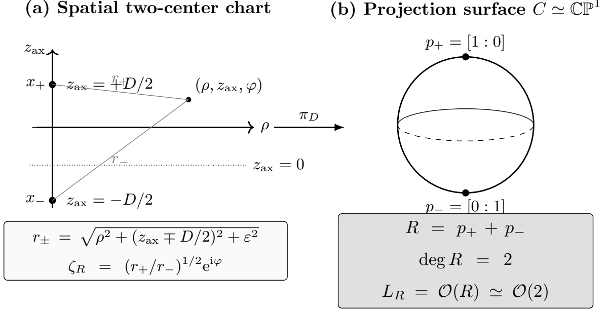
FIG. 2. Two-center projection geometry and the generation divisor. The spatial chart contains two ordered centers x_{\pm} at z_{\text{ax}} = \pm D/2 , with regulated distances r_{\pm} . The projection map \pi_D sends the regulated two-center chart to C \simeq \mathbb{CP}^1 , and in the collapsed-core limit maps the centers to the branch points p_+ and p_- . The divisor R = p_+ + p_- has degree two and defines the generation line bundle L_R = \mathcal{O}(R) \simeq \mathcal{O}(2) . The midplane normalization z_{\text{ax}} = 0 \Rightarrow |\zeta_R| = 1 fixes the residual scale of the affine coordinate.
