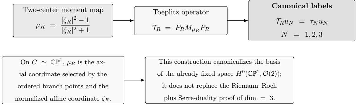
FIG. 5. Canonical family labels from the two-center Toeplitz operator. The family count \dim H^0(\mathbb{CP}^1, \mathcal{O}(2)) = 3 is basis-independent, but physical labels require a canonical Hermitian operator. The two-center projection fixes the affine coordinate \zeta_R , hence the axial moment-map function \mu_R . Projecting multiplication by \mu_R onto the protected holomorphic section space gives the Toeplitz operator \mathcal{T}_R = P_R M_{\mu_R} P_R . Its eigenvectors define the canonical generation basis, equivalent for the symmetric two-center placement to the spin-one monomial basis 1, \zeta, \zeta^2 up to normalization and ordering.
