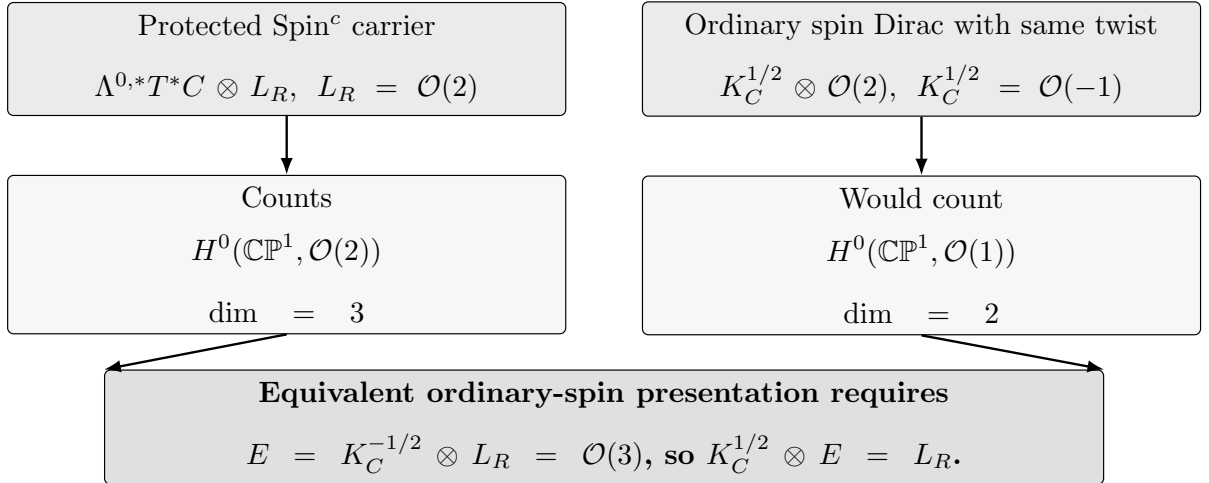
FIG. 4. Why the \text{Spin}^c Dolbeault–Dirac representative is essential. The protected sector used here is the canonical \text{Spin}^c bundle \Lambda^{0,*}T^*C twisted by L_R = \mathcal{O}(2) , and it counts H^0(\mathbb{CP}^1, \mathcal{O}(2)) , giving three positive zero modes. An ordinary spin Dirac operator on \mathbb{CP}^1 includes K_C^{1/2} = \mathcal{O}(-1) ; twisting it only by \mathcal{O}(2) would count H^0(\mathbb{CP}^1, \mathcal{O}(1)) , which is two-dimensional. Thus the \text{Spin}^c carrier is part of the stated protected sector, not an interchangeable notation.
