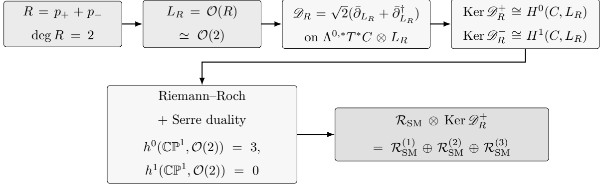
FIG. 3. \text{Spin}^c index-theoretic origin of the three protected families. The two-center divisor fixes L_R = \mathcal{O}(2) . The protected internal fermion operator is the \text{Spin}^c Dolbeault–Dirac operator, whose positive and negative kernels are identified by Hodge theory with H^0(C, L_R) and H^1(C, L_R) . For C = \mathbb{CP}^1 , Riemann–Roch and Serre duality give h^0 = 3 and h^1 = 0 , so the positive internal zero-mode space produces three four-dimensional SM chiral family copies.
