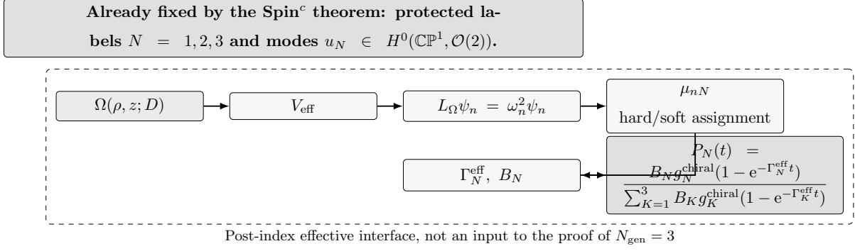
FIG. 6. Post-index scalar spectral interface for formation and visibility. After the \text{Spin}^c index theorem has fixed the protected generation space to three modes, the two-center scalar geometry supplies an effective interface for profiles, rates, and visible overlaps. The conformal factor \Omega determines V_{\text{eff}} , whose scalar eigenmodes \psi_n are connected to the protected labels only through scalarization weights and hard/soft assignment. The probability law P_N(t) describes post-index formation and visibility of N = 1, 2, 3 ; it is not an additional input to the proof of the family multiplicity.
