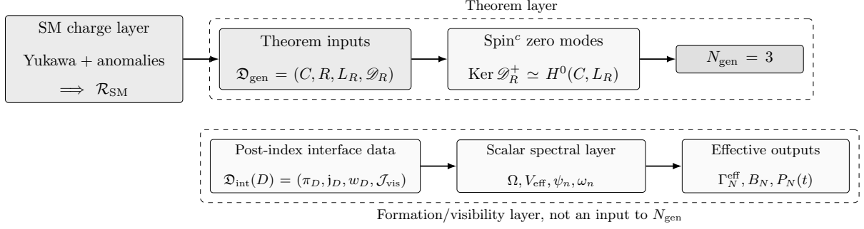
FIG. 1. Logical architecture of the PSLT Spin c generation theorem. The Standard Model charge layer fixes one anomaly-free chiral family representation \mathcal{R}_{\text{SM}} . The protected internal fermion layer uses the two-center projection data C = \mathbb{CP}^1 , R = p_+ + p_- , L_R = \mathcal{O}(R) \simeq \mathcal{O}(2) , and the Spin c Dolbeault–Dirac operator \mathcal{D}_R to prove the family multiplicity through \text{Ker } \mathcal{D}_R^+ \simeq H^0(C, L_R) . The scalar spectral, kinetic, and visibility data form a post-index effective interface and are not inputs to the theorem N_{\text{gen}} = 3 .
