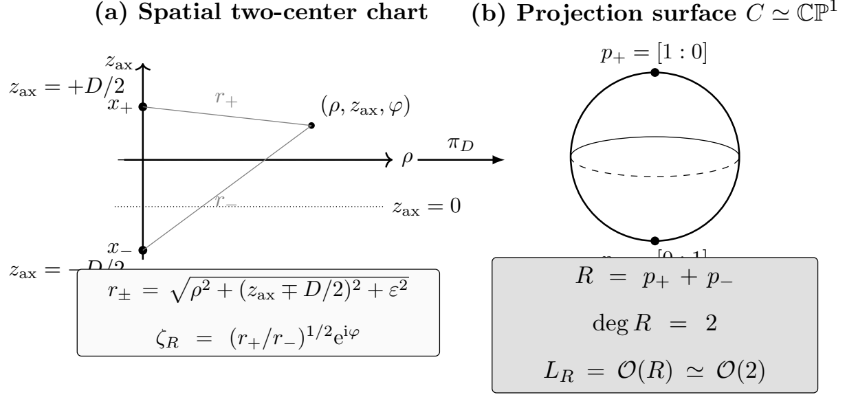
FIG. 2. Two-center projection geometry and the generation divisor. The spatial chart contains two ordered centers x_{\pm} at z_{\text{ax}} = \pm D/2 , with regulated distances r_{\pm} . The projection map \pi_D sends the regulated two-center chart to C \simeq \mathbb{CP}^1 , and in the collapsed-core limit maps the centers to the branch points p_+ and p_- . The divisor R = p_+ + p_- has degree two and defines the generation line bundle L_R = \mathcal{O}(R) \simeq \mathcal{O}(2) . The midplane normalization z_{\text{ax}} = 0 \Rightarrow |\zeta_R| = 1 fixes the residual scale of the affine coordinate.
