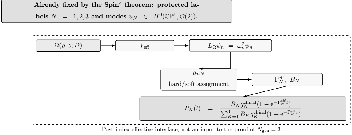
FIG. 6. Post-index scalar spectral interface for formation and visibility. After the Spin c index theorem has fixed the protected generation space to three modes, the two-center scalar geometry supplies an effective interface for profiles, rates, and visible overlaps. The conformal factor \Omega determines V_{\text{eff}} , whose scalar eigenmodes \psi_n are connected to the protected labels only through scalarization weights and hard/soft assignment. The probability law P_N(t) describes post-index formation and visibility of N = 1, 2, 3 ; it is not an additional input to the proof of the family multiplicity.
