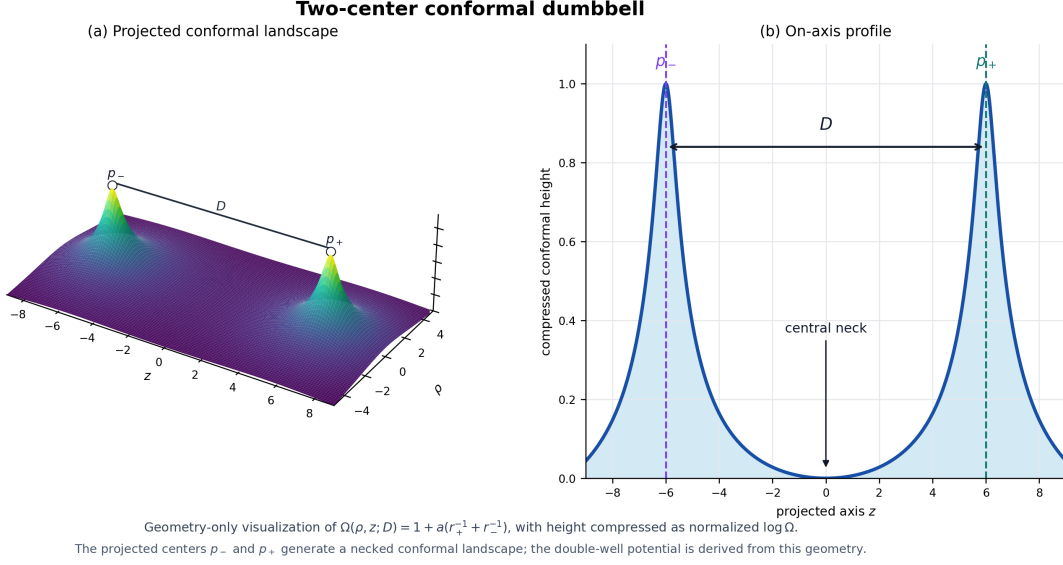
Fig. 1 Projected two-center conformal dumbbell used as the fixed background in the release closure. The figure is a physical visualization of Eq. (5), not a new independent model input.
