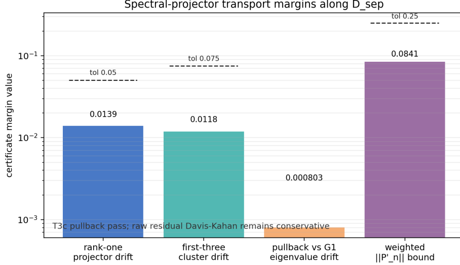
Fig. 6 Optional spectral-projector transport margins along D_{\text{sep}} . The certified object is the actual variable-box coordinate-pullback projector step; the raw residual Davis-Kahan comparator remains intentionally conservative and is not used as the pass criterion.
