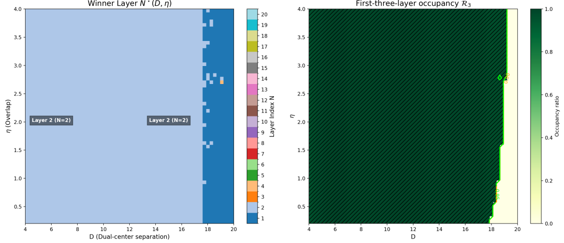
Fig. 4 Release first-three-layer occupancy map. The left panel shows the winner layer on the release scan, while the right panel shows \mathcal{R}_3 = P_1 + P_2 + P_3 . The canonical Occupancy-map parity gate requires the live plotting path to reproduce the registered fractions before the map is accepted.
