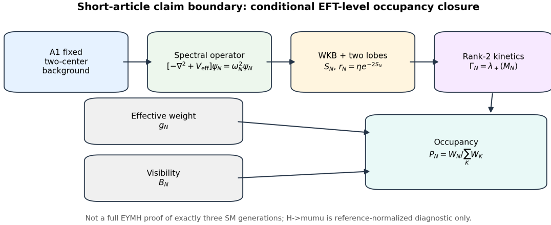
Fig. 2 Short-article closure diagram. The figure exposes the intended logical order: fixed projected background, spectral operator, WKB/two-lobe data, rank-2 kinetics, effective phase-space and visibility weights, and finally the normalized occupancy P_N . The bottom line is part of the claim boundary: this is a conditional occupancy closure, not a complete first-principles proof of exactly three SM generations.
