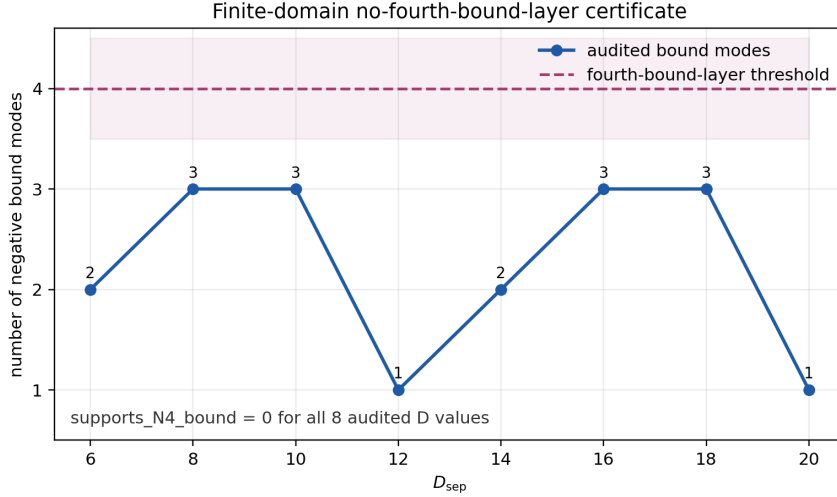
Fig. 5 Finite-domain no-fourth-bound-layer certificate. The audited single-track kinetic proxy has one to three negative bound modes over the displayed D_{\text{sep}} values, but no certified fourth bound layer. This is a finite-domain statement, not a continuum theorem.
