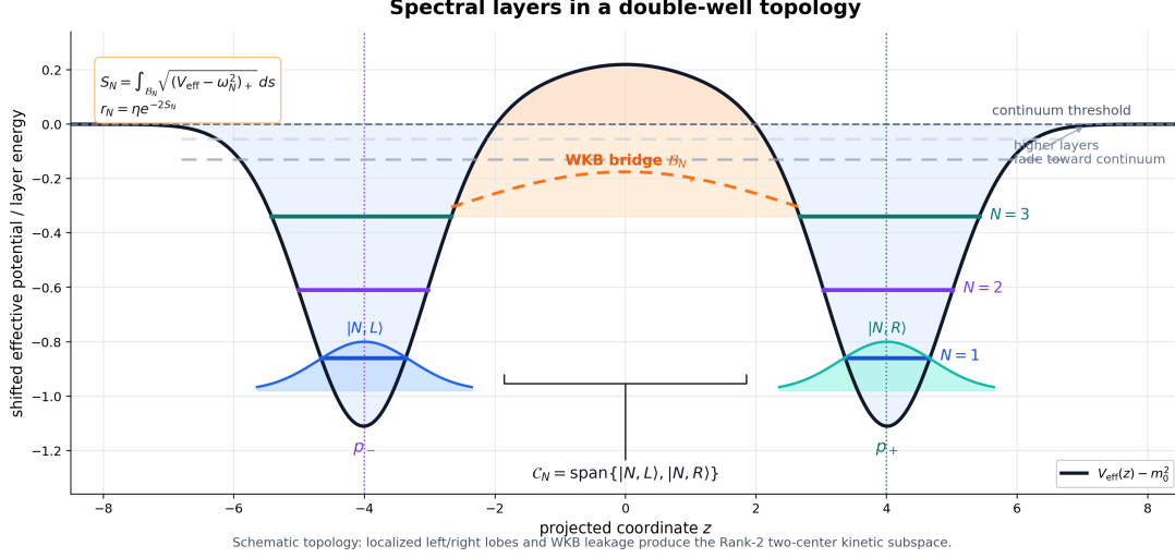
Fig. 3 Spectral layers in a double-well topology. The rank-2 matrix in Eq. (19) is the effective two-lobe description of localized modes, with WKB suppression controlled by Eq. (22).
