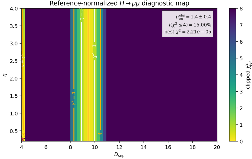
Fig. 7 Reference-normalized H \rightarrow \mu\mu diagnostic map. The color scale shows the clipped scan-level \chi^2_{\mu\mu} , the contours mark \chi^2 = 1 and \chi^2 = 4 , and the star marks the best grid point. This figure visualizes a target region only; it is not a formal global likelihood or an absolute Higgs-sector prediction.
