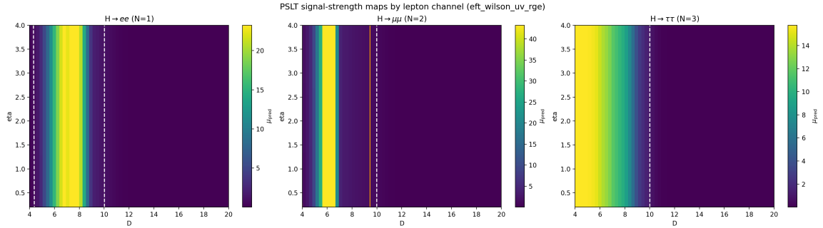
FIG. 11. PSLT EFT/Wilson-matched extension from H \rightarrow \mu\mu to three lepton channels on the same scan grid: H \rightarrow ee (left), H \rightarrow \mu\mu (middle), and H \rightarrow \tau\tau (right). Each panel shows \mu_{\ell\ell}^{\text{pred}} from Eq. (59) with the same reference-normalization point (D_0, \eta_0) = (10, 1) .
