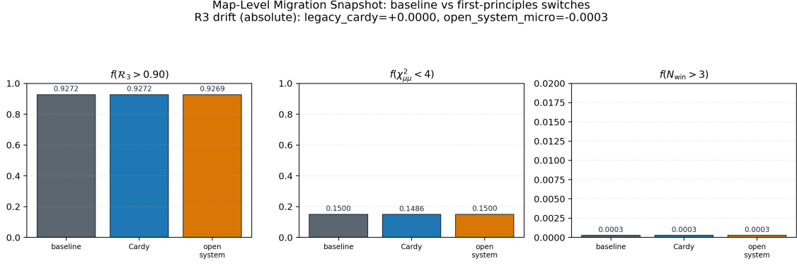
FIG. 18. Map-level migration snapshot across three scenarios. Left to right: f(\mathcal{R}_3 > 0.90) , f(\chi_{\mu\mu}^2 < 4) , and f(N_{\text{win}} > 3) .
