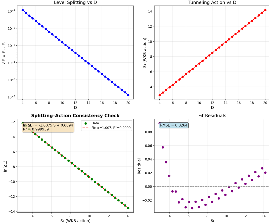
FIG. 13. Splitting-action consistency check. The level splitting \Delta E = E_2 - E_1 follows \exp(-S_1) to R^2 = 0.9999 , confirming the action-derived V_{\text{eff}} governs both spectrum and tunneling.
