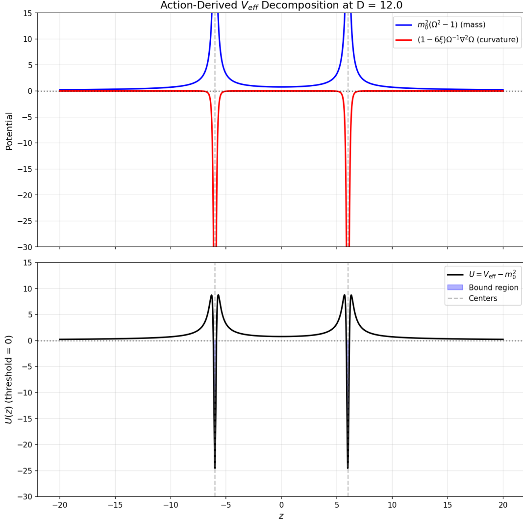
FIG. 4. Action-derived potential decomposition at D = 12 . Top: mass term m_0^2(\Omega^2 - 1) and curvature term (1 - 6\xi)\Omega^{-1}\nabla^2\Omega . Bottom: total U = V_{\text{eff}} - m_0^2 showing the double-well structure. The 4 turning points confirm the tunneling geometry.
