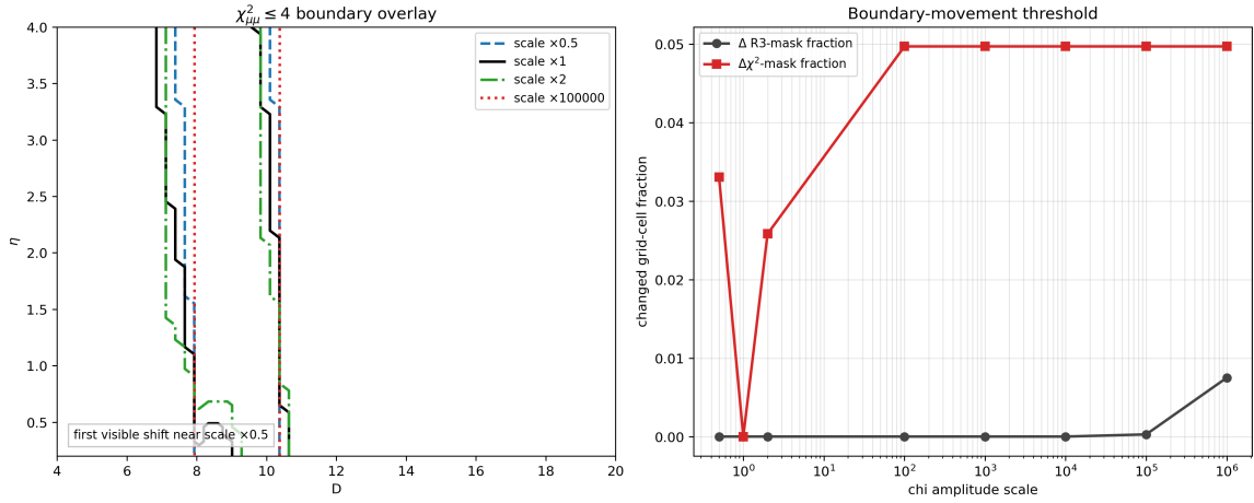
FIG. 15. Strong \chi -amplitude stress test on the global map. Left: overlay of \chi_{\mu\mu}^2 \leq 4 boundary for selected scales, including representative \times 0.5 and \times 2 stress factors. Right: changed-cell fractions versus scale (relative to baseline \times 1 ), showing early movement for the H \rightarrow \mu\mu mask and delayed movement for the \mathcal{R}_3 mask. The registered numerical certificate is indexed in the artifact registry.
