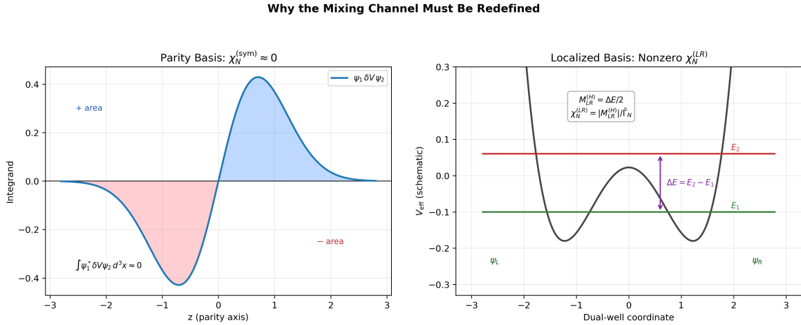
FIG. 7. Physical interpretation of the mixing channel. In the parity-symmetric basis, overlap cancellation yields \chi_N^{(\text{sym})} \approx 0 . In the localized basis, the level splitting \Delta E defines the effective coupling \chi_N^{(LR)}(D) used in the global scan.
