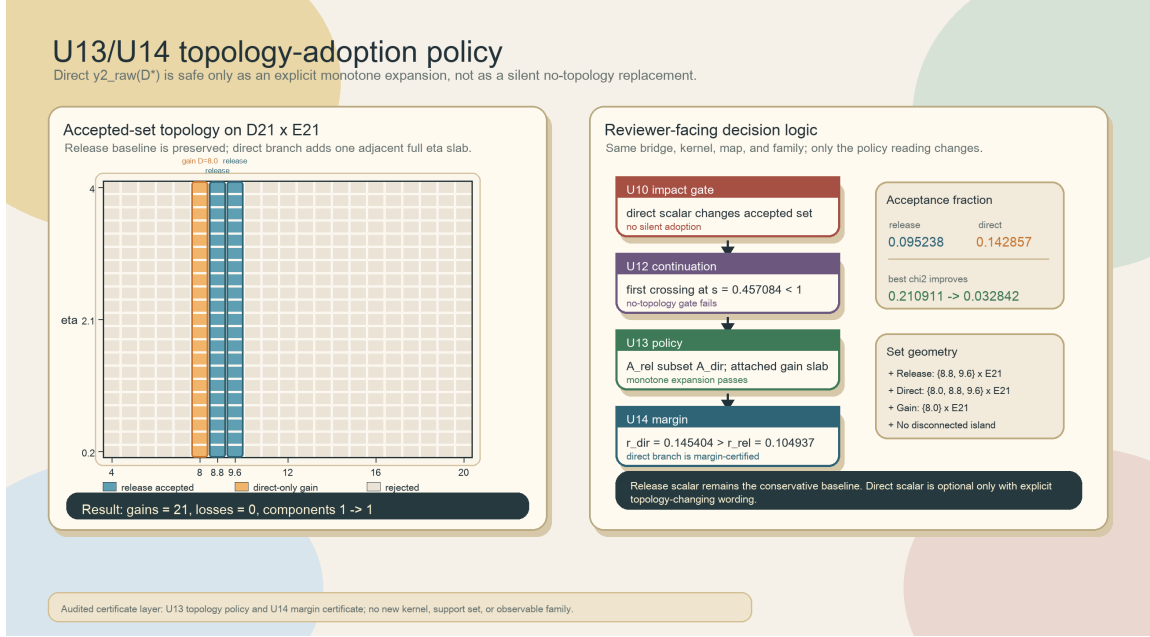
FIG. 12. Reviewer-facing U13/U14 topology-adoption policy for the direct inserted-history y_2^{\text{raw}}(D_*) scalar. Left: the accepted set grows from \{D = 8.8, 9.6\} \times E_{21} to \{D = 8.0, 8.8, 9.6\} \times E_{21} , adding one adjacent D = 8.0 slab with 21 gains, no losses, and one connected component before and after the change. Right: the decision chain separates U10's non-silent map impact, U12's no-topology obstruction, U13's monotone-expansion policy, and U14's margin certificate. The direct branch is optional and adoption-safe only with explicit topology-changing wording; the release scalar remains the conservative baseline.
