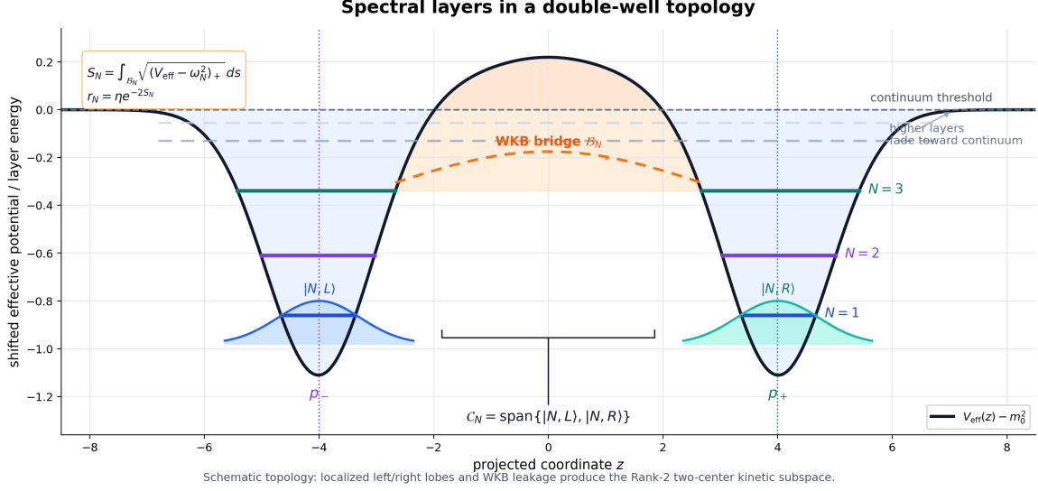
FIG. 6. Schematic topology behind the Rank-2 kinetic closure. The shifted double-well profile represents the effective two-center geometry; the low-lying layer labels N = 1, 2, 3 sit inside the wells, higher layers fade toward the continuum threshold, and the forbidden bridge \mathcal{B}_N gives the WKB action in Eq. (23). The left/right localized lobes span the two-center subspace \mathcal{C}_N = \text{span}\{|N, L\rangle, |N, R\rangle\} , explaining why the kinetic closure is naturally Rank-2 rather than an abstract matrix ansatz.
