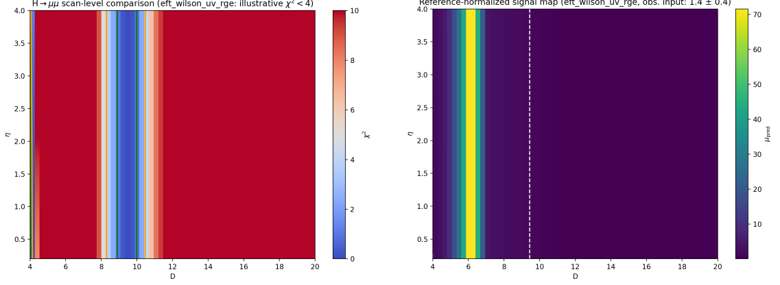
FIG. 10. Reference-normalized scan-level comparison with H \rightarrow \mu\mu under the EFT/Wilson-matched UV+LL-RG map. Left: \chi^2 map showing a restricted illustrative accepted band ( \chi^2 < 4 , equivalently p_{\text{local}} > 4.55 \times 10^{-2} for dof=1). Right: predicted \mu_{\mu\mu}^{\text{pred}} .
