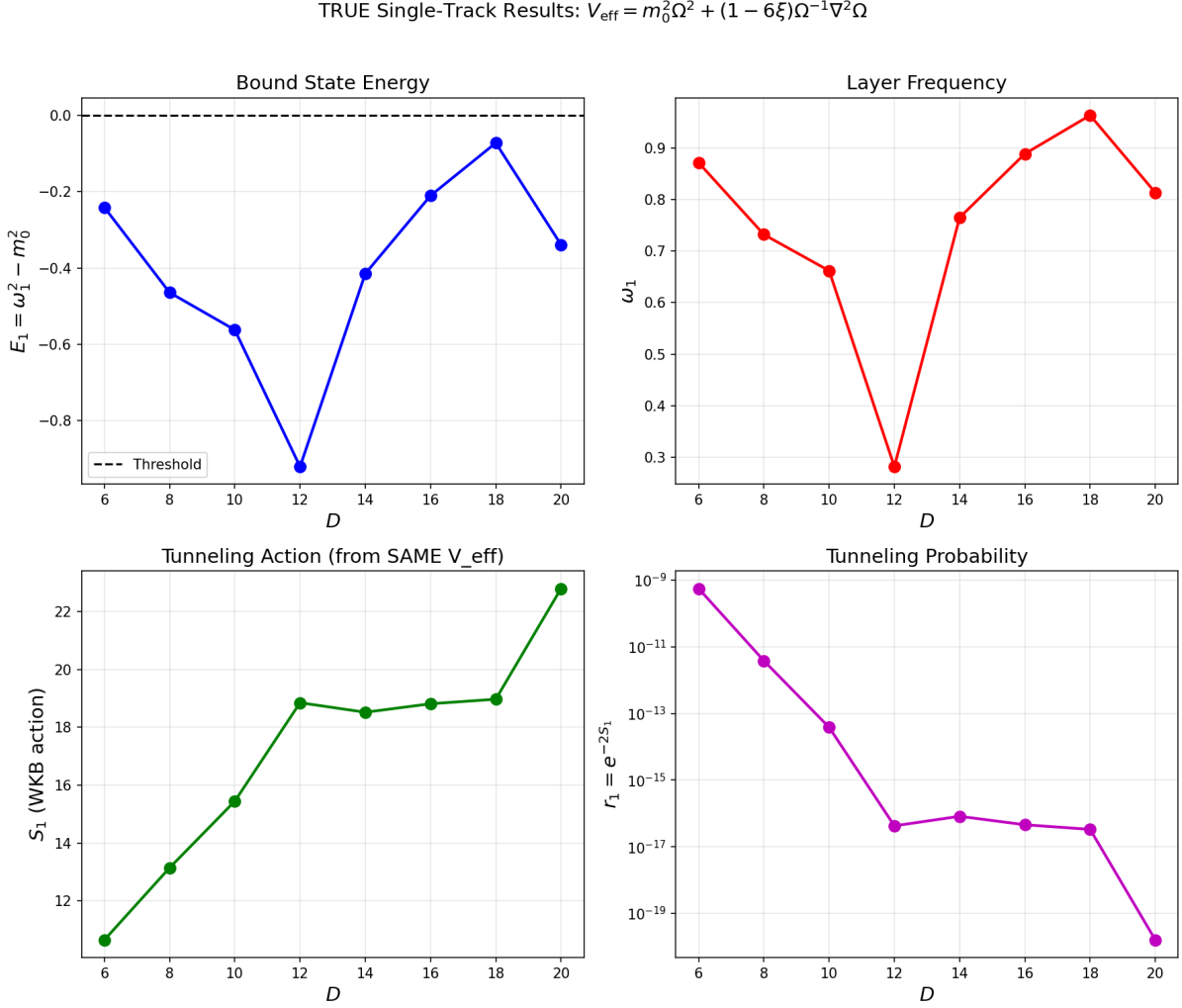
FIG. 5. Single-track results from action-derived V_{\text{eff}} . Top-left: Bound state energy E_1 < 0 . Top-right: Layer frequency \omega_1 . Bottom-left: WKB tunneling action S_1 . Bottom-right: Tunneling probability r_1 = e^{-2S_1} . All quantities are computed from the same V_{\text{eff}}(\rho, z; D) .
