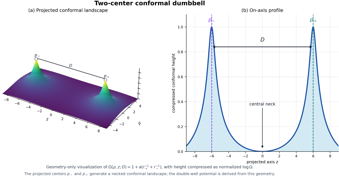
FIG. 3. Geometry-only visualization of the two-center conformal dumbbell used in the worked example. The displayed height is the normalized compressed profile \log \Omega ; it is not an additional potential term. The two projected centers p_- and p_+ generate a necked conformal landscape, from which the effective double-well potential is derived by Eq. (14).
