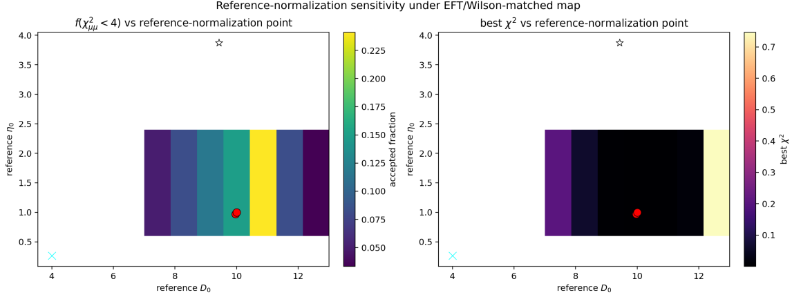
FIG. 19. Systematic sensitivity over reference-normalization points (D_0, \eta_0) under the EFT/Wilson-matched UV+LL-RG map. Left: f(\chi_{\mu\mu}^2 < 4) ; right: best \chi^2 . Overlaid markers indicate baseline fixed, \chi^2 -best, and robust-center selectors; the registered figure and data certificates are indexed in the artifact registry.
