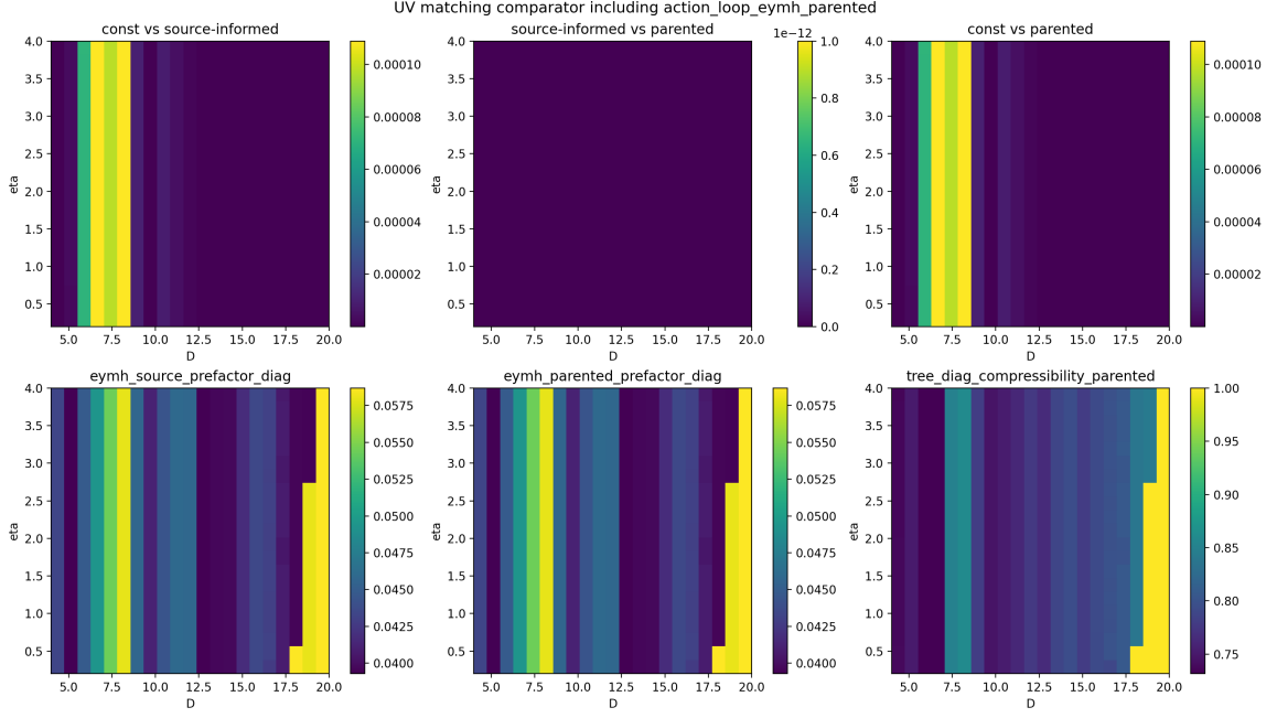
FIG. 9. EYMH-side parented finite-match comparator on the canonical D21×E21 fix grid. Top row: map-level deformation against the refreshed constant baseline and the source-informed comparator; the source-informed and parented maps coincide to numerical precision. Bottom row: the corresponding EYMH source prefactor, parented prefactor, and tree-diagonal compressibility witness.
