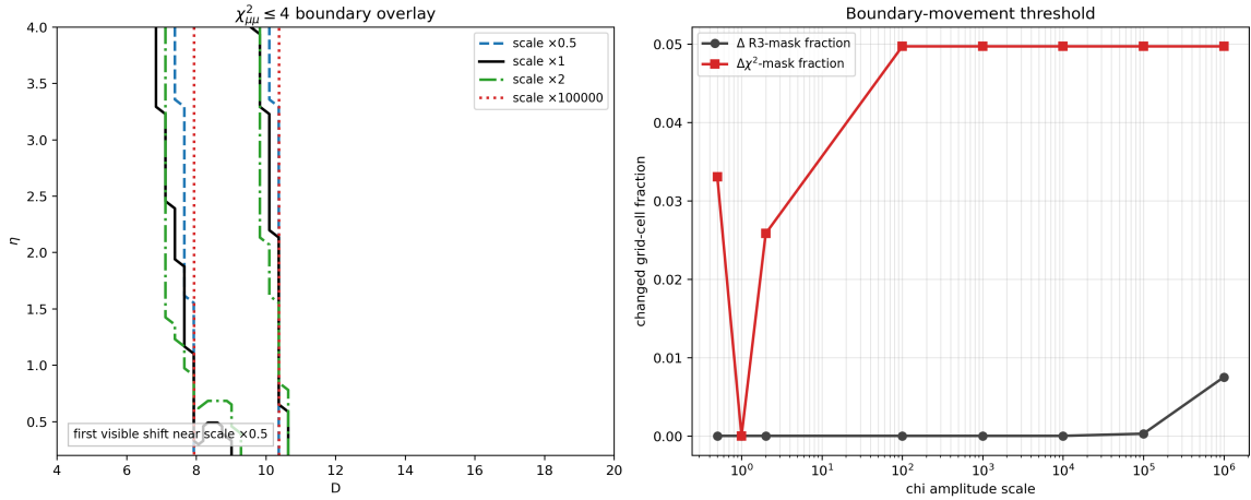
FIG. 13. Strong \chi -amplitude stress test on the global map. Left: overlay of \chi_{\mu\mu}^2 \leq 4 boundary for selected scales, including representative \times 0.5 and \times 2 stress factors. Right: changed-cell fractions versus scale (relative to baseline \times 1 ), showing early movement for the H \rightarrow \mu\mu mask and delayed movement for the \mathcal{R}_3 mask. The registered numerical certificate is indexed in the artifact registry.
