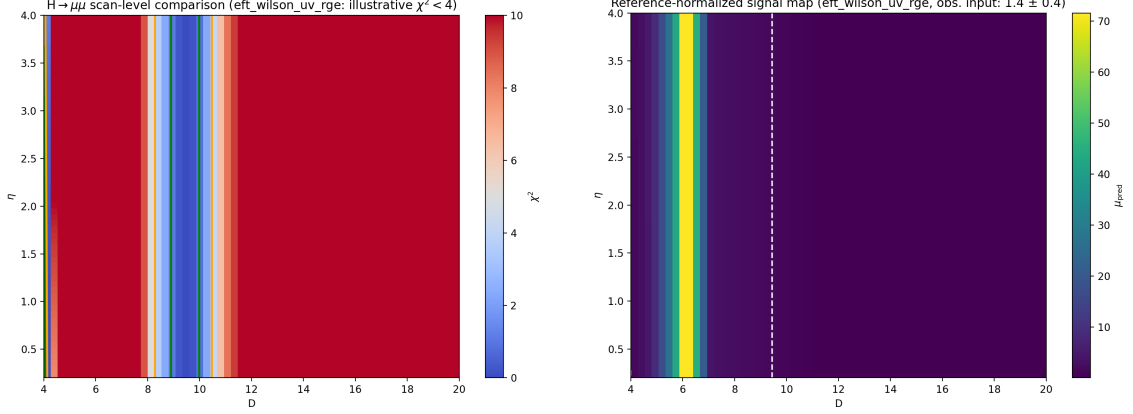
FIG. 8. Reference-normalized scan-level comparison with H \rightarrow \mu\mu under the EFT/Wilson-matched UV+LL-RG map. Left: \chi^2 map showing a restricted illustrative accepted band ( \chi^2 < 4 , equivalently p_{\text{local}} > 4.55 \times 10^{-2} for dof=1). Right: predicted \mu_{\mu\mu}^{\text{pred}} .
