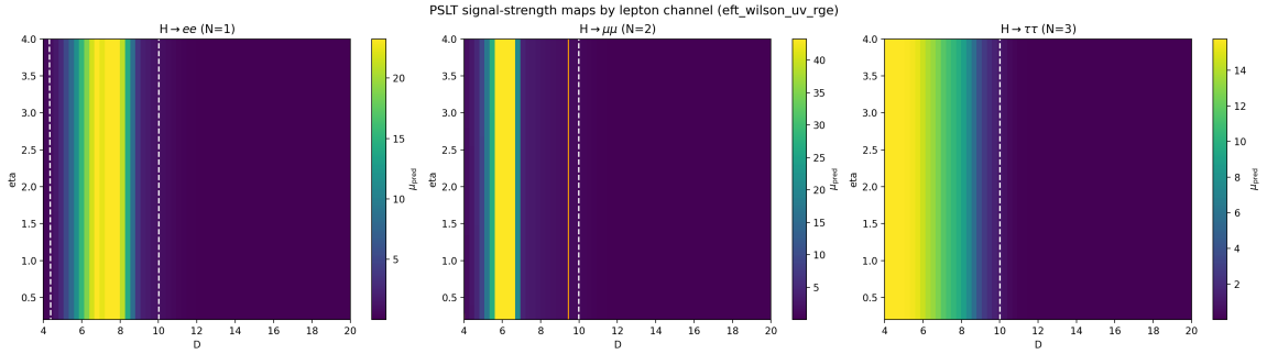
FIG. 9. PSLT EFT/Wilson-matched extension from H \rightarrow \mu\mu to three lepton channels on the same scan grid: H \rightarrow ee (left), H \rightarrow \mu\mu (middle), and H \rightarrow \tau\tau (right). Each panel shows \mu_{\ell\ell}^{\text{pred}} from Eq. (56) with the same reference-normalization point (D_0, \eta_0) = (10, 1) .
