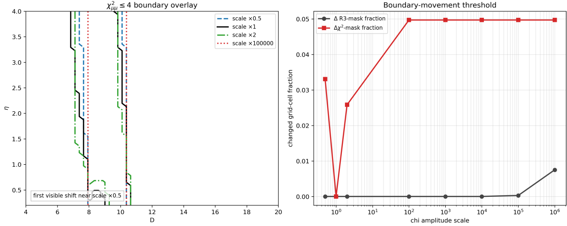
FIG. 12. Strong \chi -amplitude stress test on the global map. Left: overlay of \chi^2_{\mu\mu} \leq 4 boundary for selected scales, including the requested \times 0.5 and \times 2 . Right: changed-cell fractions versus scale (relative to baseline \times 1 ), showing early movement for the H \rightarrow \mu\mu mask and delayed movement for the \mathcal{R}_3 mask. Source data file: output/chi_fp_2d/chi_scale_stress_test.csv .
