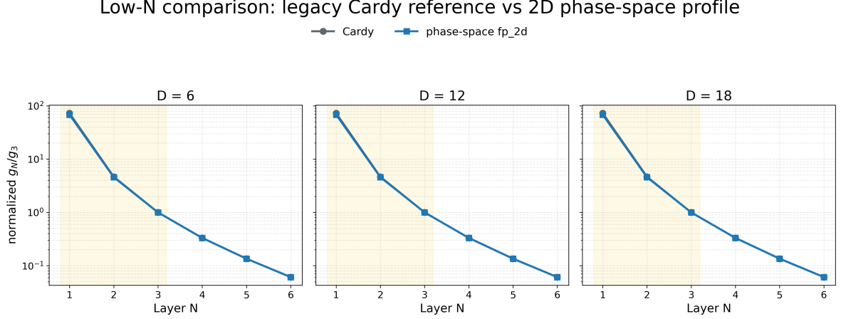
FIG. 13. Low- N comparison between legacy Cardy reference and 2D phase-space profile on D = \{6, 12, 18\} , shown as normalized ratios g_N/g_3 (log scale). The highlighted band marks N = 1, 2, 3 . Source files: paper/gn_cardy_vs_phase_space.png , paper/gn_cardy_vs_phase_space.csv .
