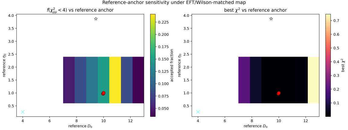
FIG. 14. Systematic sensitivity over reference-normalization points (D_0, \eta_0) under the EFT/Wilson-matched UV+LL-RG map. Left: f(\chi_{\mu\mu}^2 < 4) ; right: best \chi^2 . Overlaid markers indicate baseline fixed, \chi^2 -best, and robust-center selectors. Source files: paper/reference_anchor_sensitivity.csv , paper/reference_anchor_sensitivity.png .
