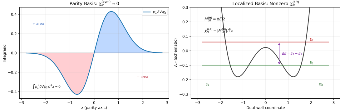
FIG. 5. Physical interpretation of the mixing channel. In the parity-symmetric basis, overlap cancellation yields \chi_N^{(\text{sym})} \approx 0 . In the localized basis, the level splitting \Delta E defines the effective coupling \chi_N^{(LR)}(D) used in the global scan.
