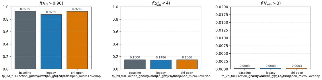
FIG. 13. Map-level migration snapshot across three scenarios. Left to right: f(\mathcal{R}_3 > 0.90) , f(\chi^2_{\mu\mu} < 4) , and f(N_{\text{win}} > 3) .
