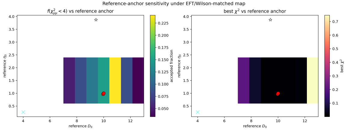
FIG. 16. Systematic sensitivity over reference-normalization points (D_0, \eta_0) under the EFT/Wilson-matched UV+LL-RG map. Left: f(\chi_{\mu\mu}^2 < 4) ; right: best \chi^2 . Overlaid markers indicate baseline fixed, \chi^2 -best, and robust-center selectors. Source files: paper/reference_anchor_sensitivity.csv , paper/reference_anchor_sensitivity.png .
