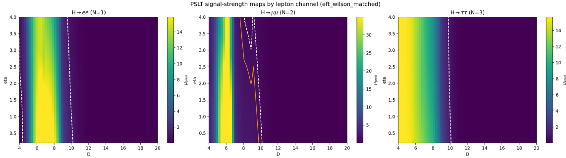
FIG. 8. PSLT EFT/Wilson-matched extension from H \rightarrow \mu\mu to three lepton channels on the same scan grid: H \rightarrow ee (left), H \rightarrow \mu\mu (middle), and H \rightarrow \tau\tau (right). Each panel shows \mu_{\ell\ell}^{\text{pred}} from Eq. (51) with the same reference point (D_0, \eta_0) = (10, 1) .
