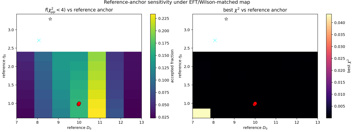
FIG. 14. Systematic sensitivity over reference anchors (D_0, \eta_0) under the EFT/Wilson-matched map. Left: f(\chi_{\mu\mu}^2 < 4) ; right: best \chi^2 . Overlaid markers indicate baseline fixed, \chi^2 -best, and robust-center selectors. Source files: paper/reference_anchor_sensitivity.csv , paper/reference_anchor_sensitivity.png .
