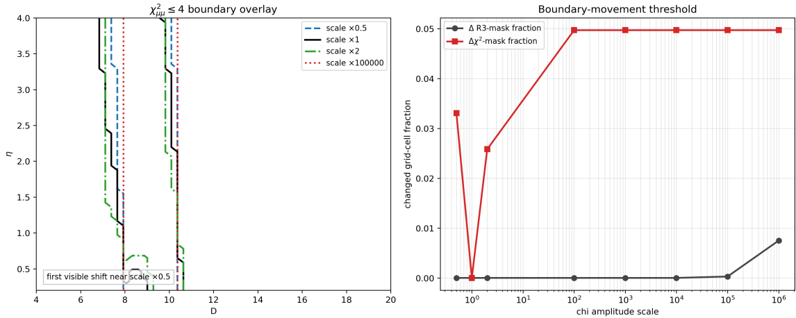
FIG. 11. Strong \chi -amplitude stress test on the global map. Left: overlay of \chi_{\mu\mu}^2 \leq 4 boundary for selected scales, including the requested \times 0.5 and \times 2 . Right: changed-cell fractions versus scale (relative to baseline \times 1 ), showing early movement for the H \rightarrow \mu\mu mask and delayed movement for the \mathcal{R}_3 mask. Source data file: output/chi_fp_2d/chi_scale_stress_test.csv .
