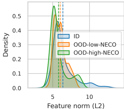
(C) Feature Norm Distribution
