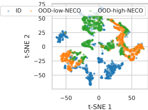
(A) Feature Geometry (t-SNE)
