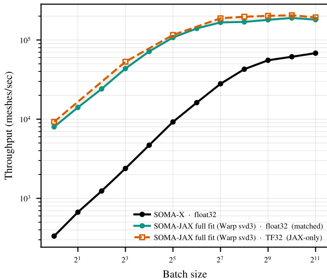
Throughput — float32 is the only fair pair
