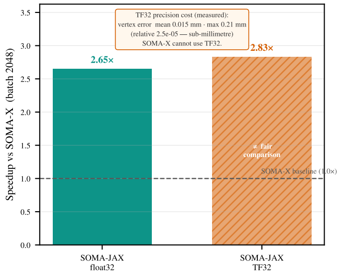
What TF32 buys, and what it costs
