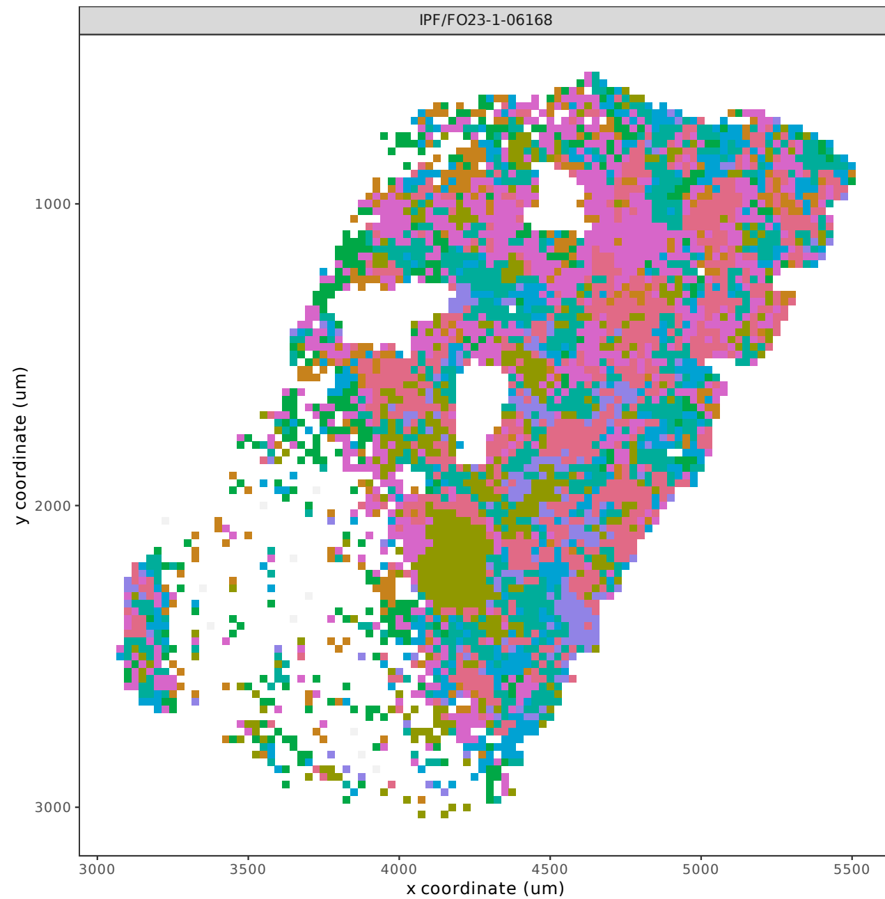
IPF/FO23-1-06168: K=8 spatial niche assignment Disease group: IPF; evaluable Bin50: 3955; Bin50 size: 25 x 25 um
