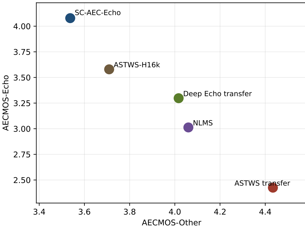
(a) Blind AECMOS operating point
